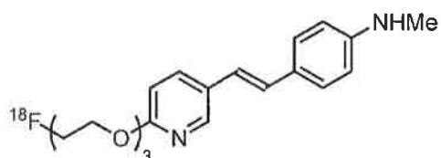
[^{18}\text{F}]\text{florbetapir} (clogP = 3.52)
