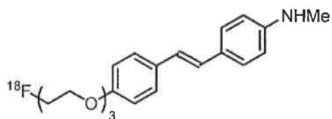
[^{18}\text{F}]\text{florbetaben} (clogP = 4.12)
