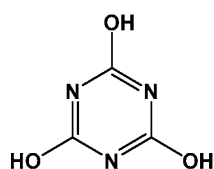
Formula (IIa) (cyanuric acid)
