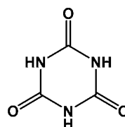
Formula (IIb) (isocyanuric acid)
