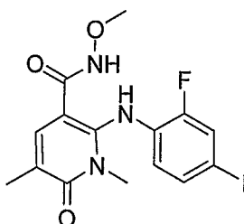
2-(2-fluoro-4-iodophenylamino)-N-methoxy-1,5-dimethyl-6-oxo-1,6-dihydropyridine-3-carboxamide
