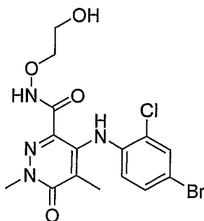
4-(4-bromo-2-chlorophenylamino)-N-(2-hydroxyethoxy)-1,5-dimethyl-6-oxo-1,6-dihydropyridazine-3-carboxamide
