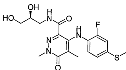
(S)-N-(2,3-Dihydroxypropyl)-4-(2-fluoro-4-(methylthio)phenylamino)-1,5-dimethyl-6-oxo-1,6-dihydropyridazine-3-carboxamide
