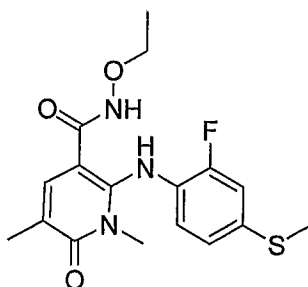
N-ethoxy-2-(2-fluoro-4-(methylthio)phenylamino)-1,5-dimethyl-6-oxo-1,6-dihydropyridine-3-carboxamide
