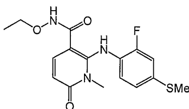
N-ethoxy-2-(2-fluoro-4-(methylthio)phenylamino)-1-methyl-6-oxo-1,6-dihydropyridine-3-carboxamide.
