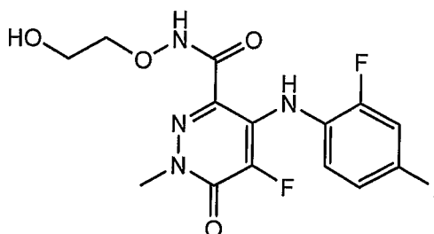
5-Fluoro-4-(2-fluoro-4-iodophenylamino)-N-(2-hydroxyethoxy)-1-methyl-6-oxo-1,6-dihydropyridazine-3-carboxamide
