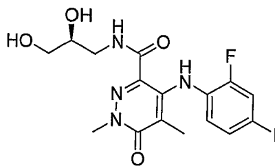
(S)-N-(2,3-Dihydroxypropyl)-4-(2-fluoro-4-iodophenylamino)-1,5-dimethyl-6-oxo-1,6-dihydropyridazine-3-carboxamide
