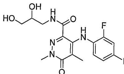
N-(2,3-Dihydroxypropyl)-4-(2-fluoro-4-iodophenylamino)-1,5-dimethyl-6-oxo-1,6-dihydropyridazine-3-carboxamide
