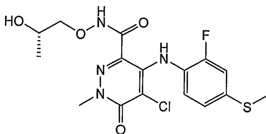
(S)-5-Chloro-4-(2-fluoro-4-(methylthio)phenylamino)-N-(2-hydroxypropoxy)-1-methyl-6-oxo-1,6-dihydropyridazine-3-carboxamide
