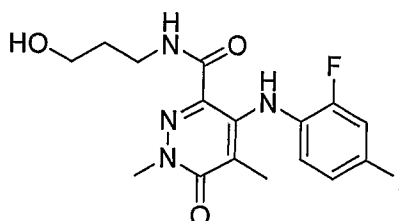
4-(2-Fluoro-4-iodophenylamino)-N-(3-hydroxypropyl)-1,5-dimethyl-6-oxo-1,6-dihydropyridazine-3-carboxamide
