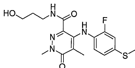
4-(2-Fluoro-4-(methylthio)phenylamino)-N-(3-hydroxypropyl)-1,5-dimethyl-6-oxo-1,6-dihydropyridazine-3-carboxamide
