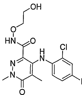
4-(2-chloro-4-iodophenylamino)-N-(2-hydroxyethoxy)-1,5-dimethyl-6-oxo-1,6-dihydropyridazine-3-carboxamide
