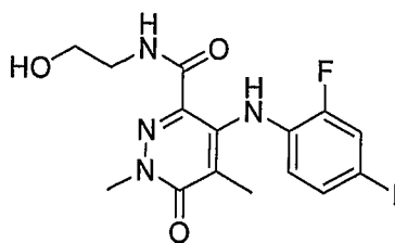
4-(2-Fluoro-4-iodophenylamino)-N-(2-hydroxyethyl)-1,5-dimethyl-6-oxo-1,6-dihydropyridazine-3-carboxamide
