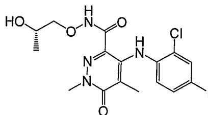
(S)-4-(2-chloro-4-iodophenylamino)-N-(2-hydroxypropoxy)-1,5-dimethyl-6-oxo-1,6-dihydropyridazine-3-carboxamide
