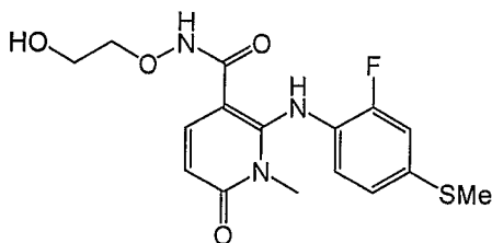
2-(2-fluoro-4-(methylthio)phenylamino)-N-(2-hydroxyethoxy)-1-methyl-6-oxo-1,6-dihydropyridine-3-carboxamide
