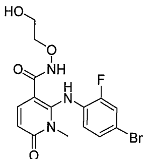
2-(4-bromo-2-fluorophenylamino)-N-(2-hydroxyethoxy)-1-methyl-6-oxo-1,6-dihydropyridine-3-carboxamide
