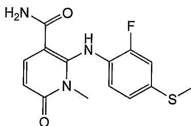
2-(2-fluoro-4-(methylthio)phenylamino)-1-methyl-6-oxo-1,6-dihydropyridine-3-carboxamide
