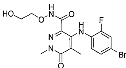
4-(4-Bromo-2-fluorophenylamino)-N-(2-hydroxyethoxy)-1,5-dimethyl-6-oxo-1,6-dihydropyridazine-3-carboxamide
