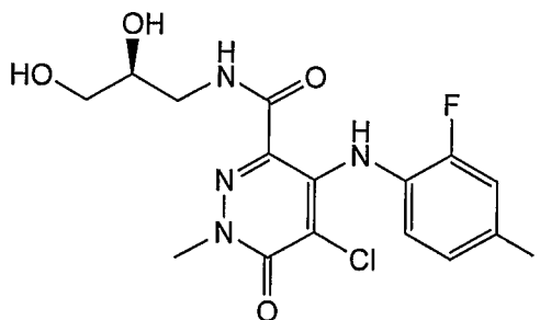
(S)-5-Chloro-N-(2,3-dihydroxypropyl)-4-(2-fluoro-4-iodophenylamino)-1-methyl-6-oxo-1,6-dihydropyridazine-3-carboxamide
