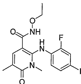
N-ethoxy-2-(2-fluoro-4-iodophenylamino)-1,5-dimethyl-6-oxo-1,6-dihydropyridine-3-carboxamide
