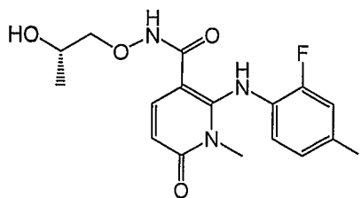
(S)-2-(2-fluoro-4-iodophenylamino)-N-(2-hydroxypropoxy)-1-methyl-6-oxo-1,6-dihydropyridine-3-carboxamide
