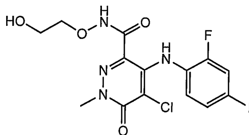
5-Chloro-4-(2-fluoro-4-iodophenylamino)-N-(2-hydroxyethoxy)-1-methyl-6-oxo-1,6-dihydropyridazine-3-carboxamide
