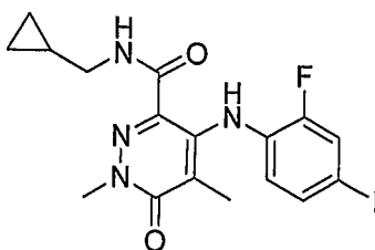
N-(Cyclopropylmethyl)-4-(2-fluoro-4-iodophenylamino)-1,5-dimethyl-6-oxo-1,6-dihydropyridazine-3-carboxamide
