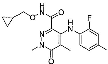
N-(Cyclopropylmethoxy)-4-(2-fluoro-4-iodophenylamino)-1,5-dimethyl-6-oxo-1,6-dihydropyridazine-3-carboxamide
