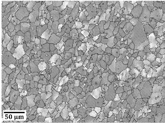
(a) Alloy of the Invention
