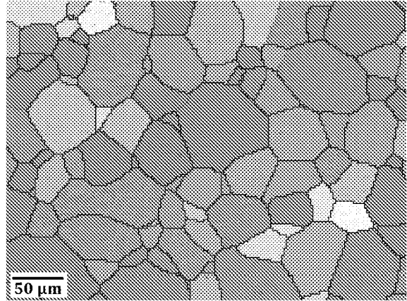
(b) Standard Beta-C Alloy
