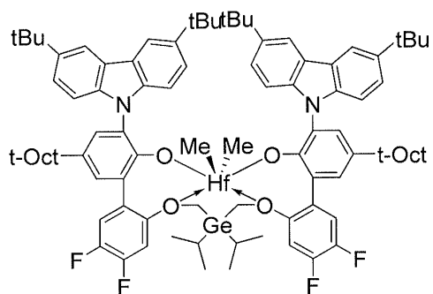
Procatalyst 3
