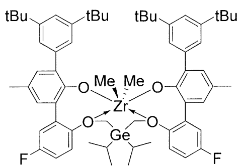
Procatalyst 6
