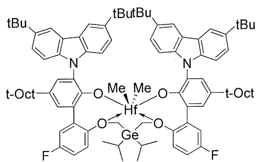
Procatalyst 2
