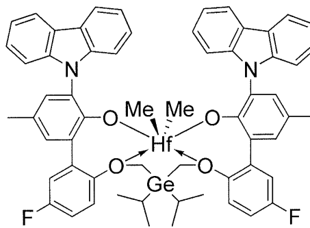
Procatalyst 4
