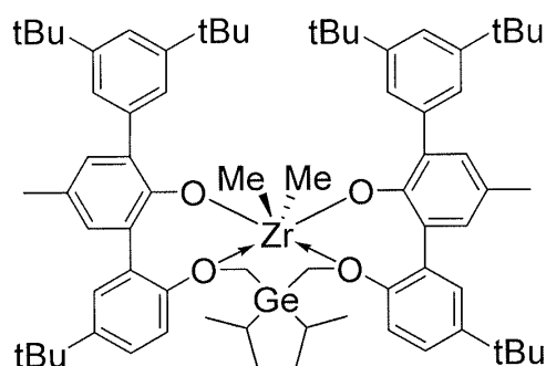
Procatalyst 7
