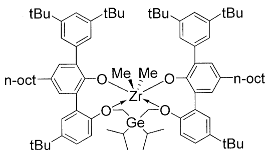
Procatalyst 9
