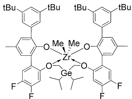
Procatalyst 5
