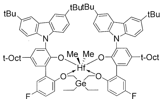
Procatalyst 1
