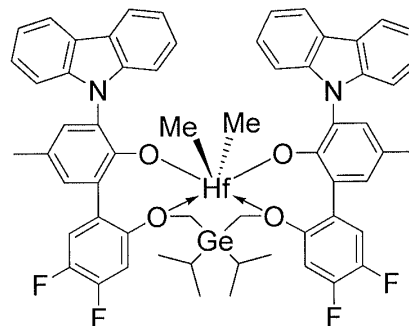
Procatalyst 8
