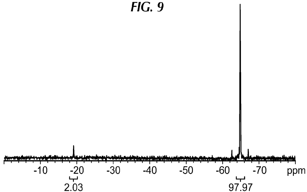
^{119}\text{Sn} NMR of Isopropyl tris(dimethylamino)tin Synthesized at About -40°C
