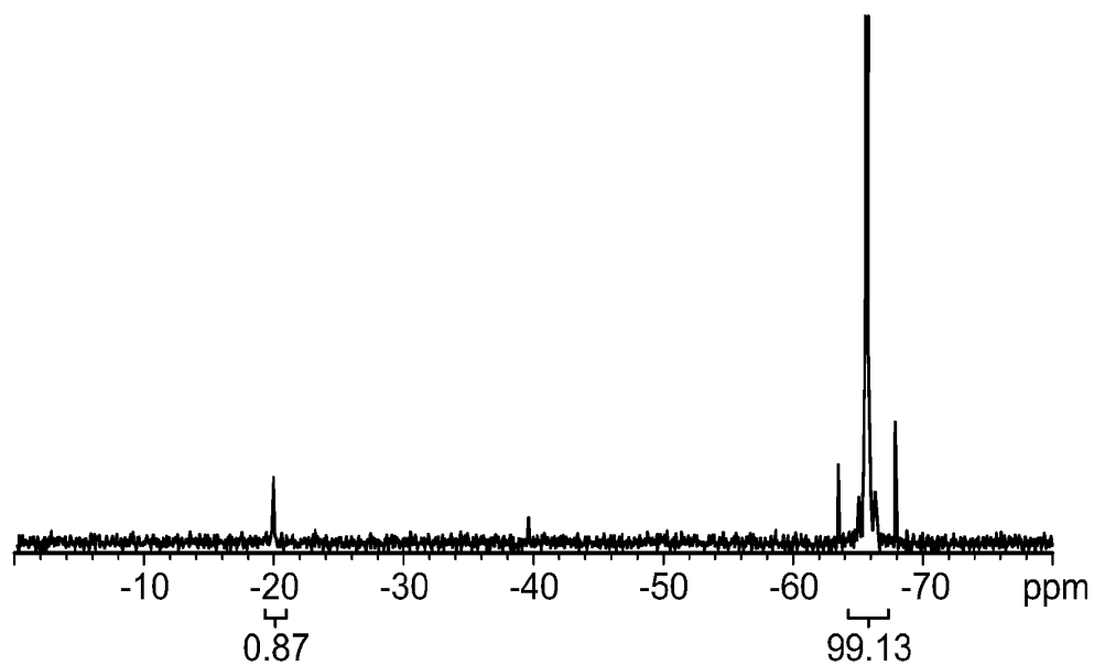
^{119}\text{Sn} NMR of Isopropyl tris(dimethylamino)tin Synthesized at About 0°C
