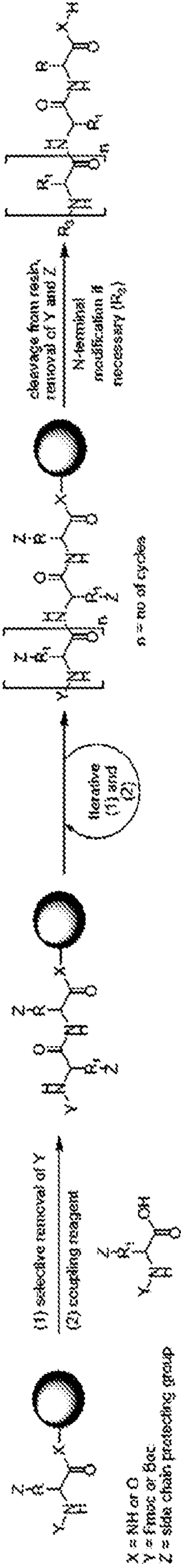
Sequential synthesis strategy by Solid Phase Peptide Synthesis (SPPS)
