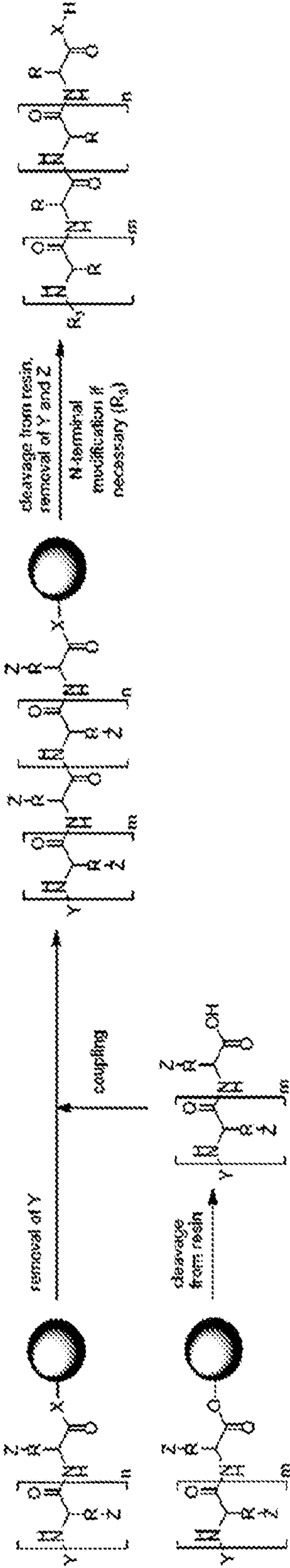
Convergent synthesis strategy by Solid Phase Peptide Synthesis (SPPS)
