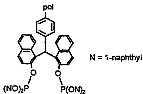
Supported Ligand SL42
