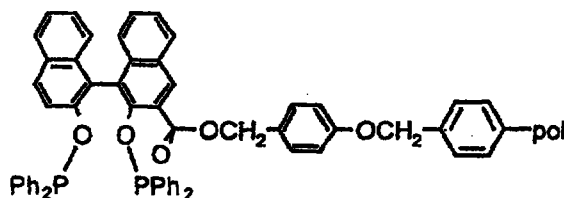
Supported Ligand SL29
