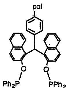
Supported Ligand SL 41
