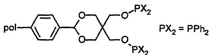
Supported Ligand SL1
