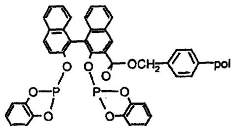
Supported Ligand SL45
