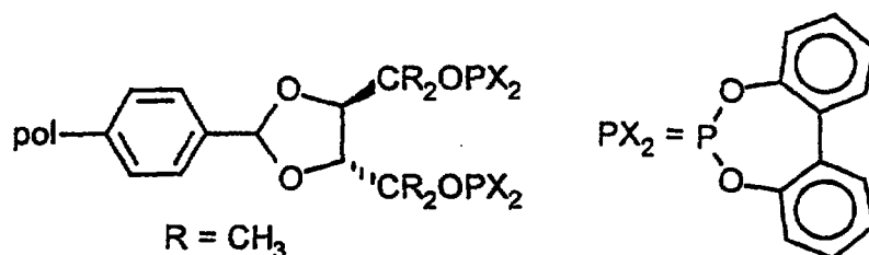
Supported Ligand SL6
