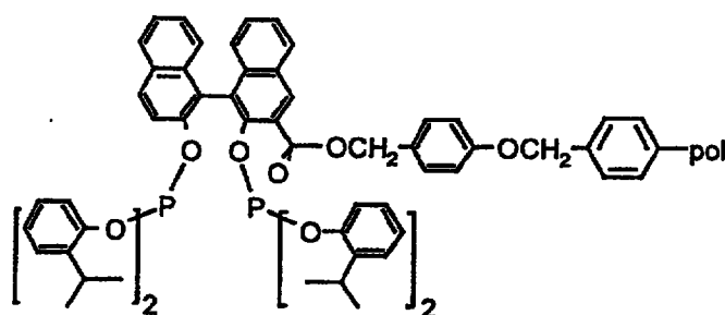
Supported Ligand SL31
