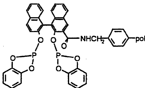
Supported Ligand SL27
