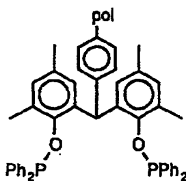
Supported Ligand SL55
