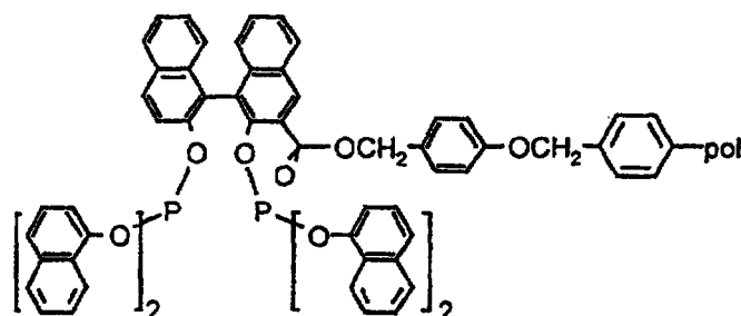
Supported Ligand SL32
