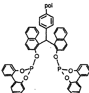
Supported Ligand SL39
