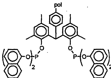
Supported Ligand SL54
