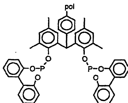
Supported Ligand SL51
