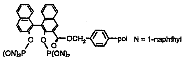
Supported Ligand SL46
