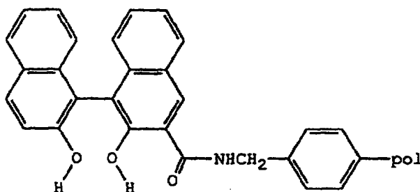
SD10 Supported diol SD10
