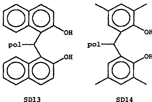
Supported Diol SD13
