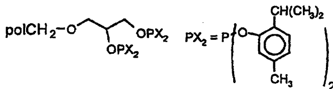
Supported Ligand SL16
