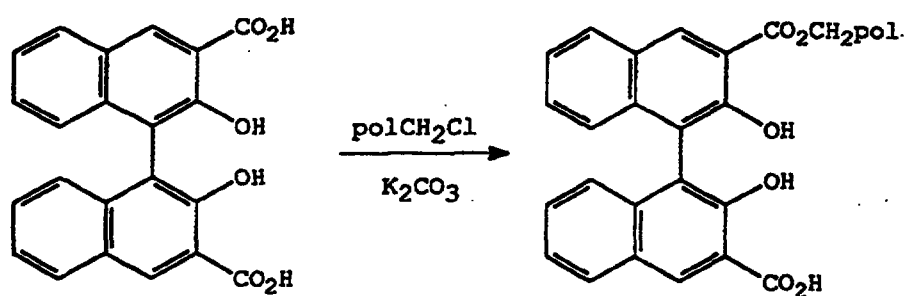
Supported Diol SD14
