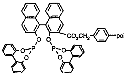
Supported Ligand SL34
