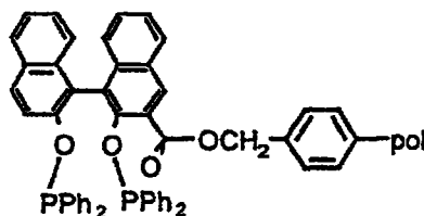
Supported Ligand SL35
