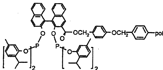
Supported Ligand SL30
