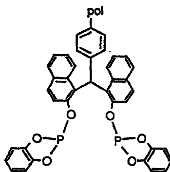
Supported Ligand SL40
