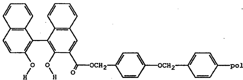
SD11 Supported Diol SD11
