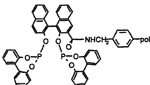
Supported Ligand SL23
