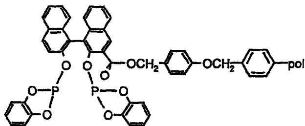
Supported Ligand SL33
