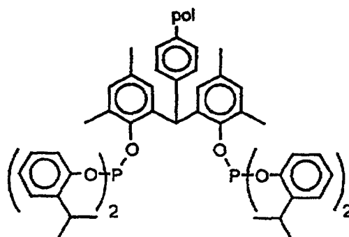
Supported Ligand SL52
