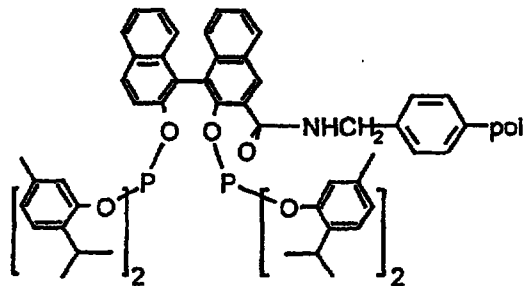
Supported Ligand SL24
