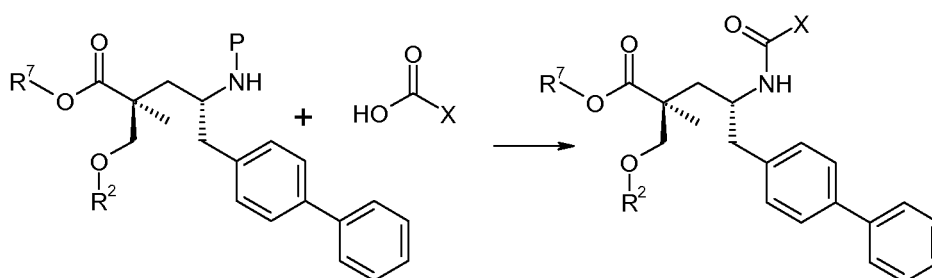
Scheme IV
