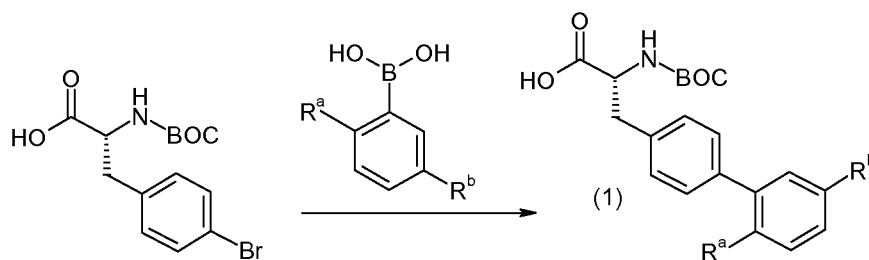
Scheme V
