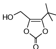
Scheme II
