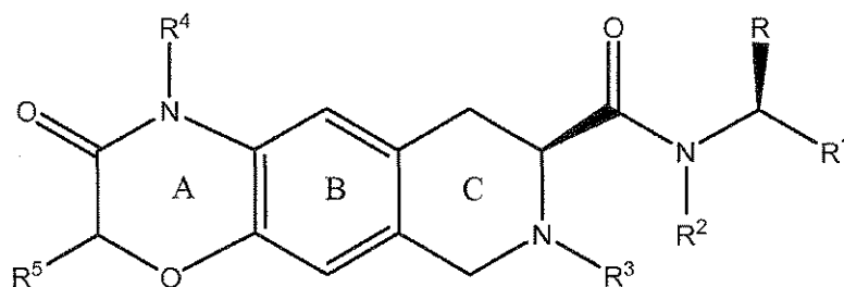
Formula (I-A)
