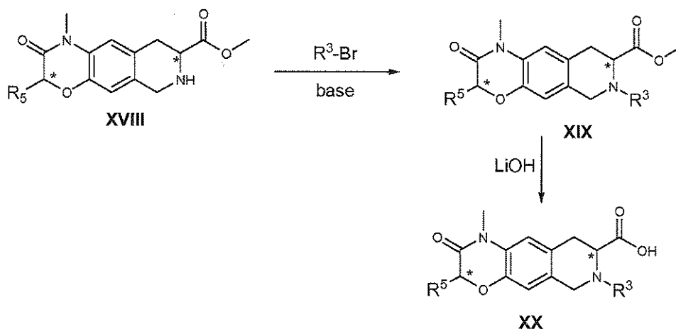
Scheme 2
