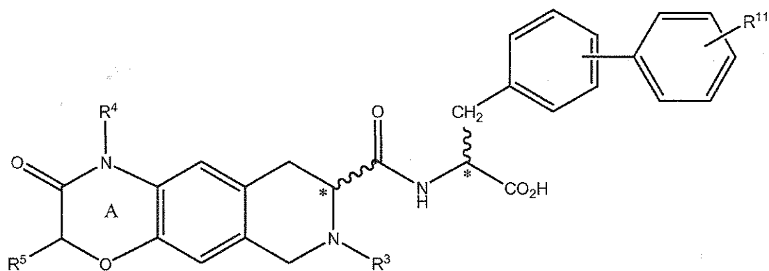
Formula (I-E)
