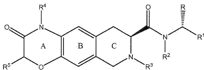
Formula (I-D)
