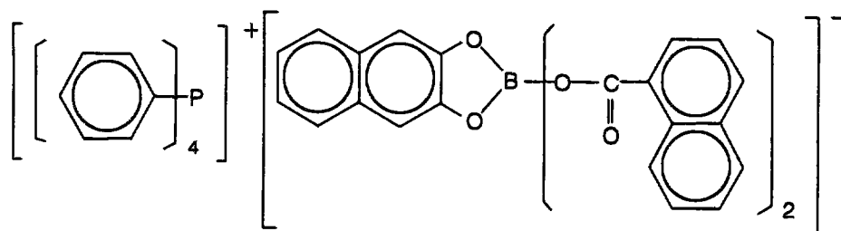
Compound 8
