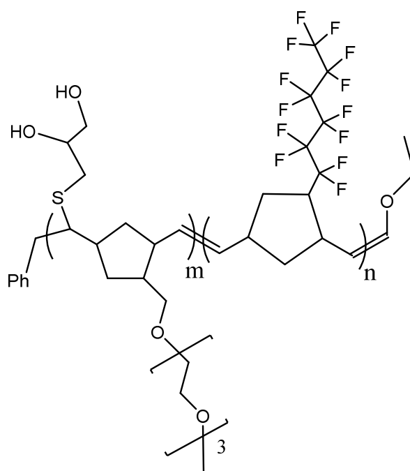
or Poly(NTEG-b-NPF6)/Thioglycerol
