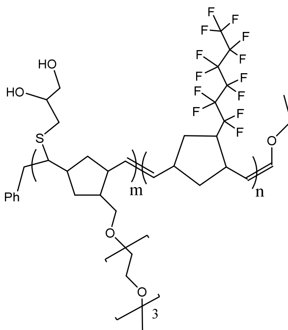
or Poly(NTEG-b-NPF6)/Thioglycerol
