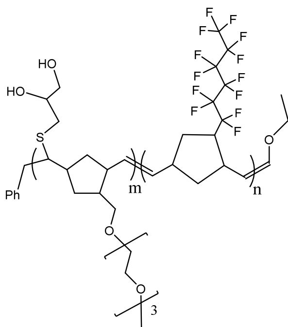
Poly(NTEG-b-NPF6)/Thioglycerol
