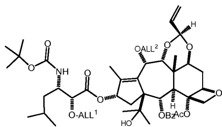
ALLMC of a 10-alpha abeo-taxane analog (19e)
