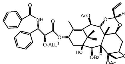
ALLMC of a 10-beta taxane analog (19b)
