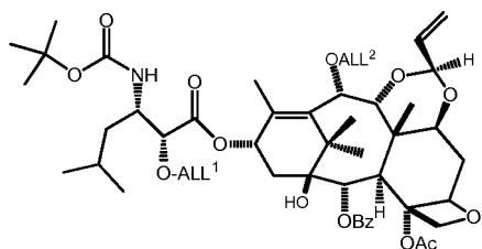
ALLMC of a 10-alpha taxane analog (19c)
