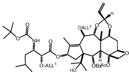
ALLMC of a 10-beta abeo-taxane analog (19g)
