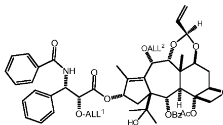
ALLMC of a 10-alpha abeo-taxane analog (19f)
