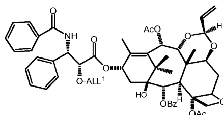
ALLMC of a 10-alpha analog (19d)
