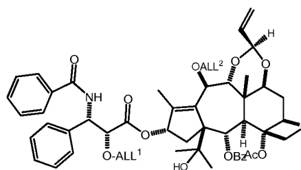
ALLMC of a 10-beta abeo-taxane analog (19h)
