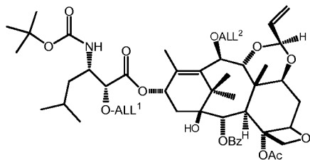
ALLMC of a 10-beta-taxane analog (19a)
