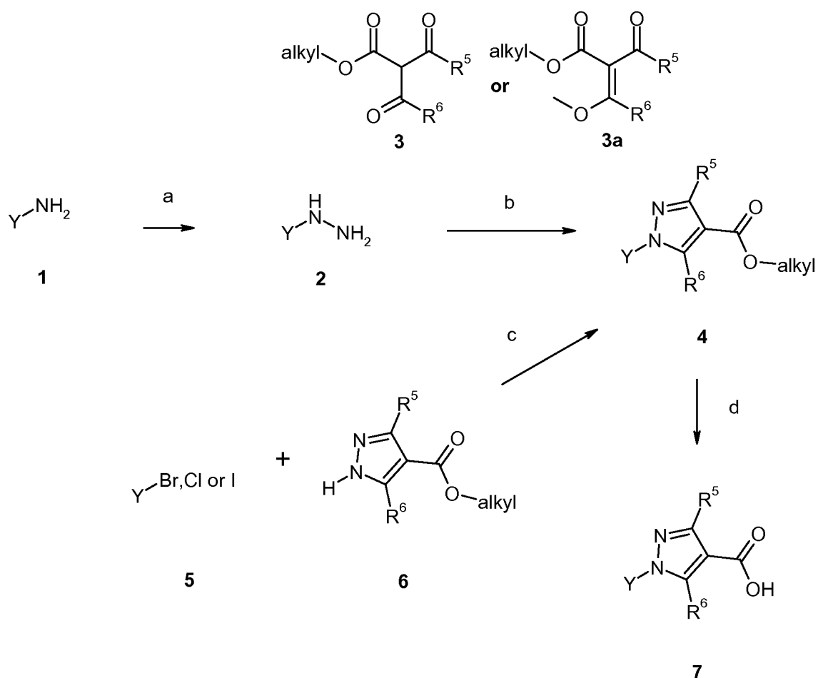
Scheme 1
