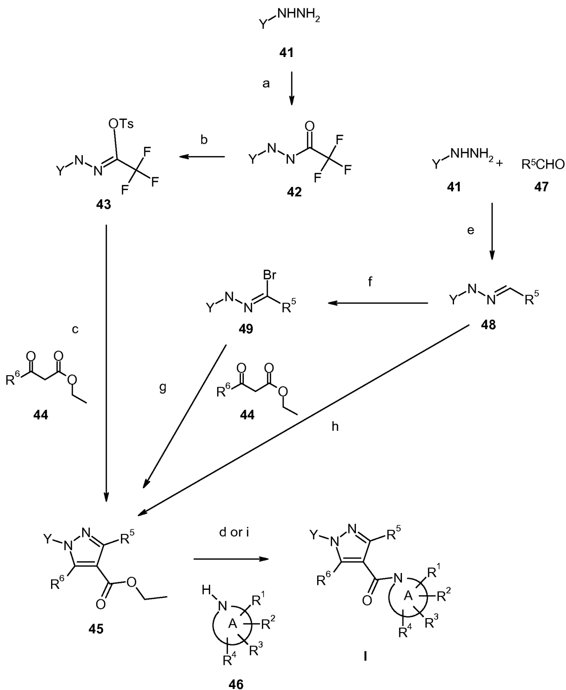
Scheme 5
