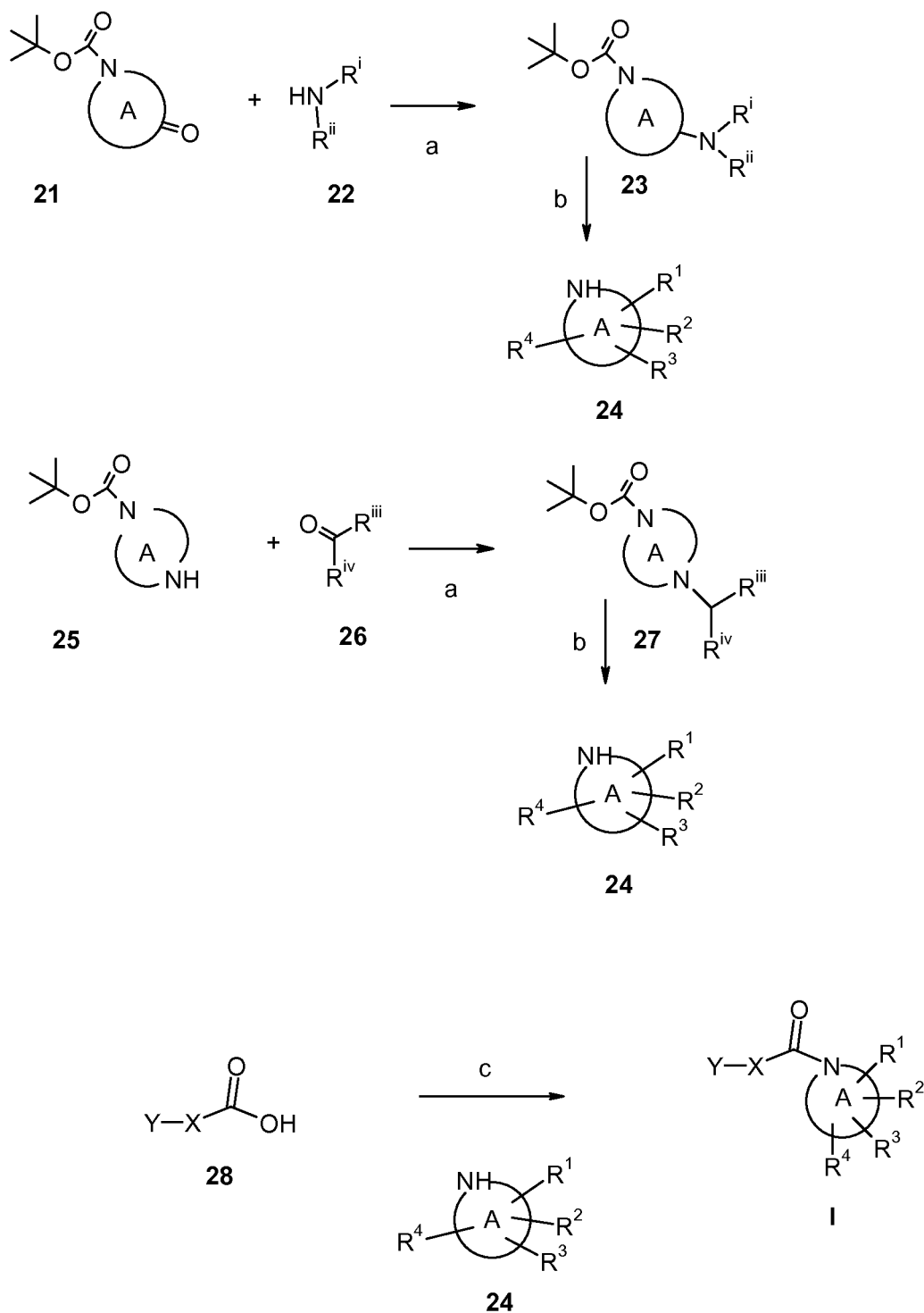
Scheme 3
