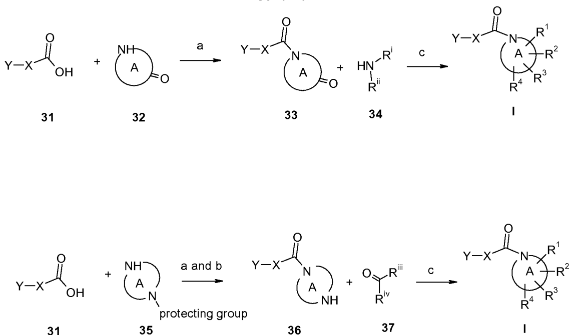
Scheme 4
