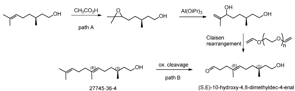
Figure 1: Synthetic scheme for the preparation of the compound of formula (I)
