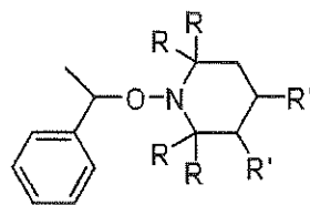
NOR Regulator
