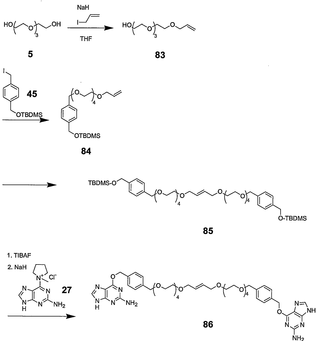
Scheme 18
