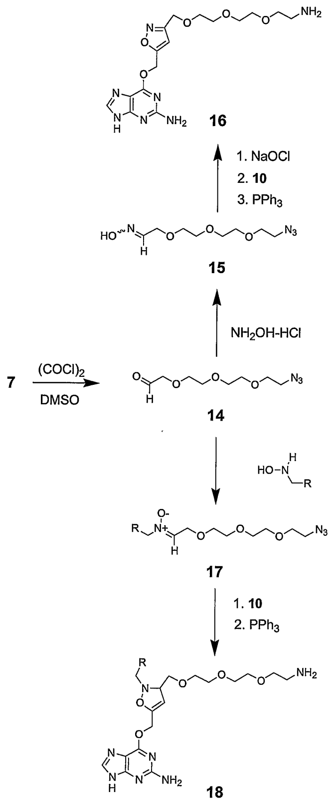
Scheme 2
