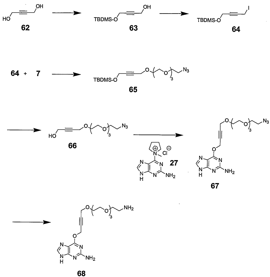
Scheme 13
