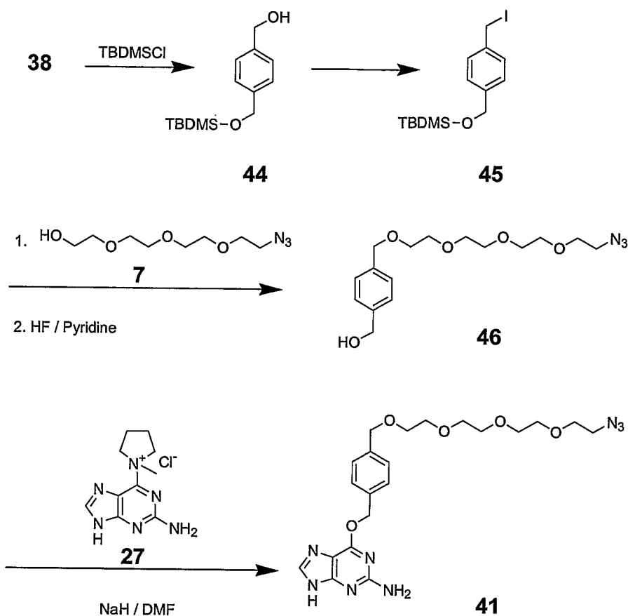
Scheme 8
