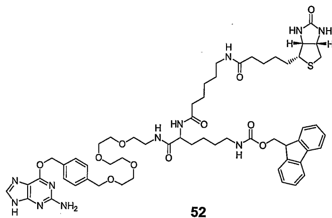
Scheme 9 (continued)
