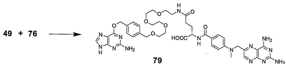
Scheme 16
