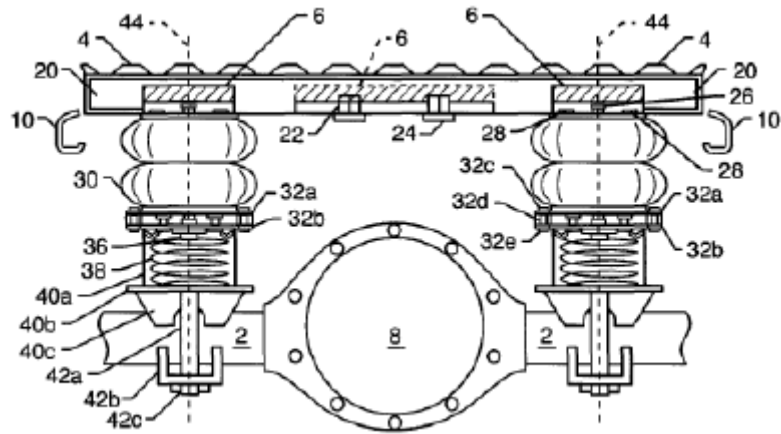
PRIOR ART [US7959174]
