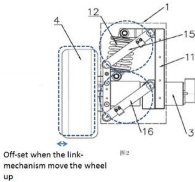
PRIOR ART [CN206106867U]
