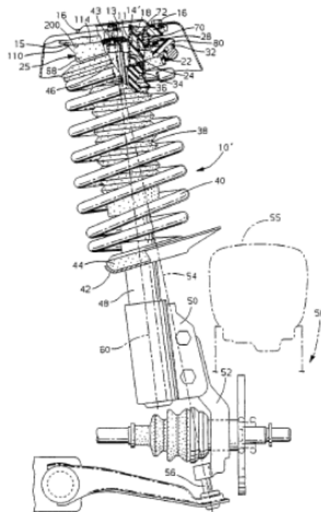
PRIOR ART [US5454585]
