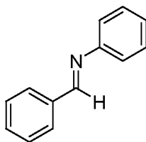
Imine A
