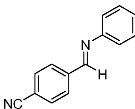
Cyano-imine B
