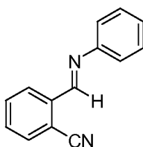
Cyano-imine A
