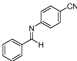
Cyano-imine C
