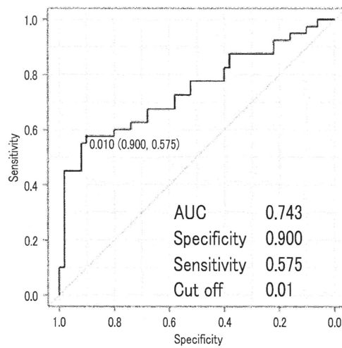
rBC2-Gal3BP
