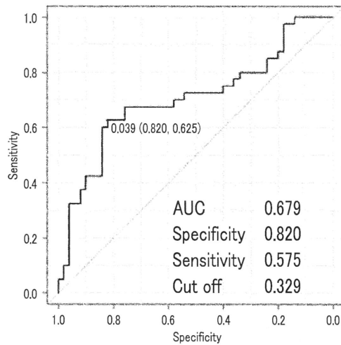
rBC2-Gal3BP
