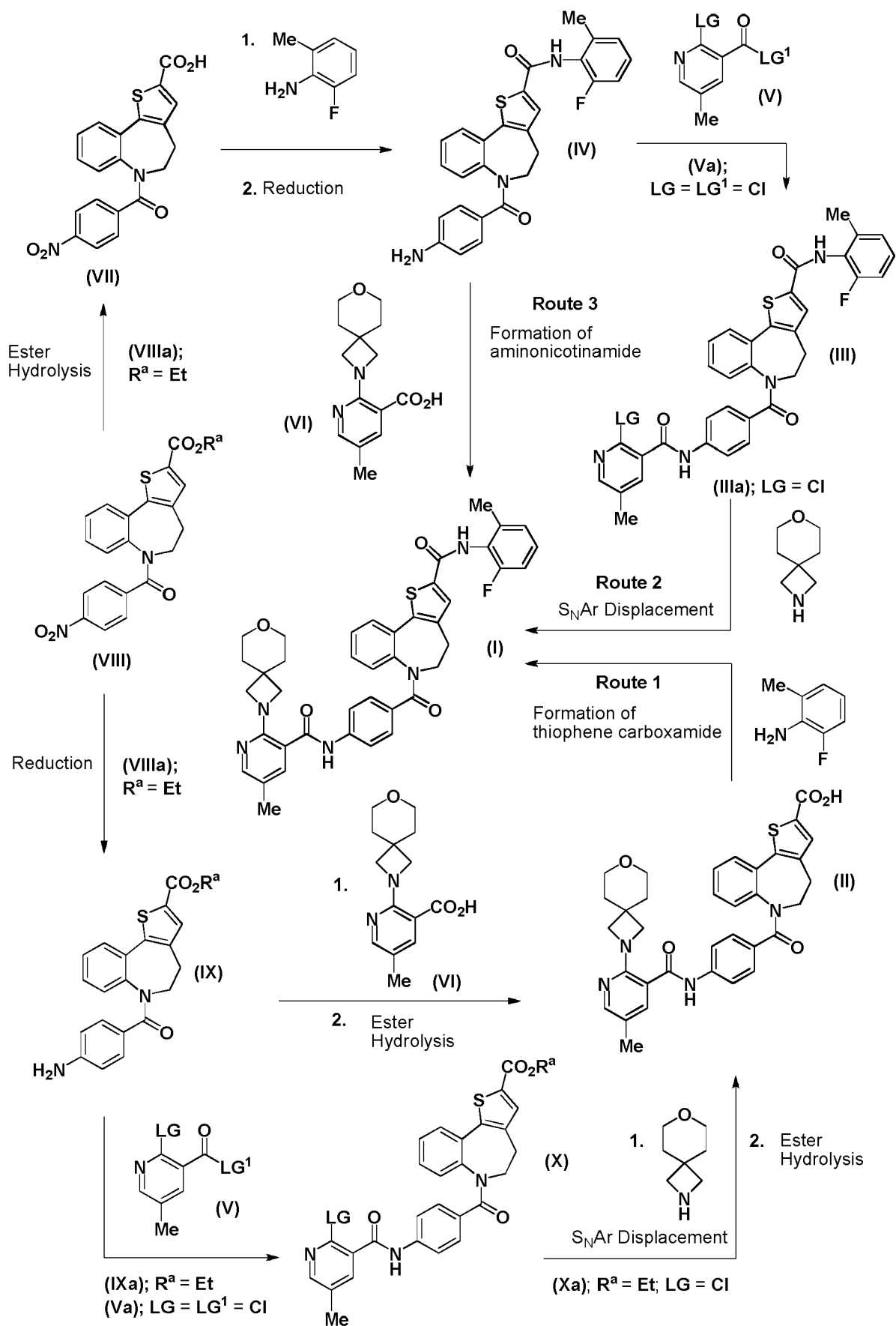
Scheme 1: Synthetic routes used for the preparation of Compound (I).
