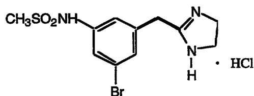
N-[3-Bromo-5-(4,5-dihydro-1H-imidazol-2-ylmethyl)-phenyl]-methanesulfonamide hydrochloride
