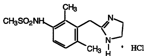
N-[3-(4,5-dihydro-1H-imidazol-2-ylmethyl)-2,4-dimethyl-phenyl]-methanesulfonamide hydrochloride
