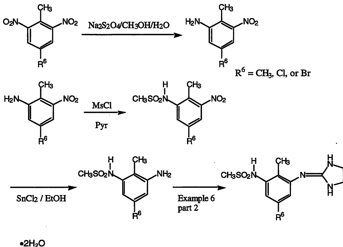
Scheme Q
