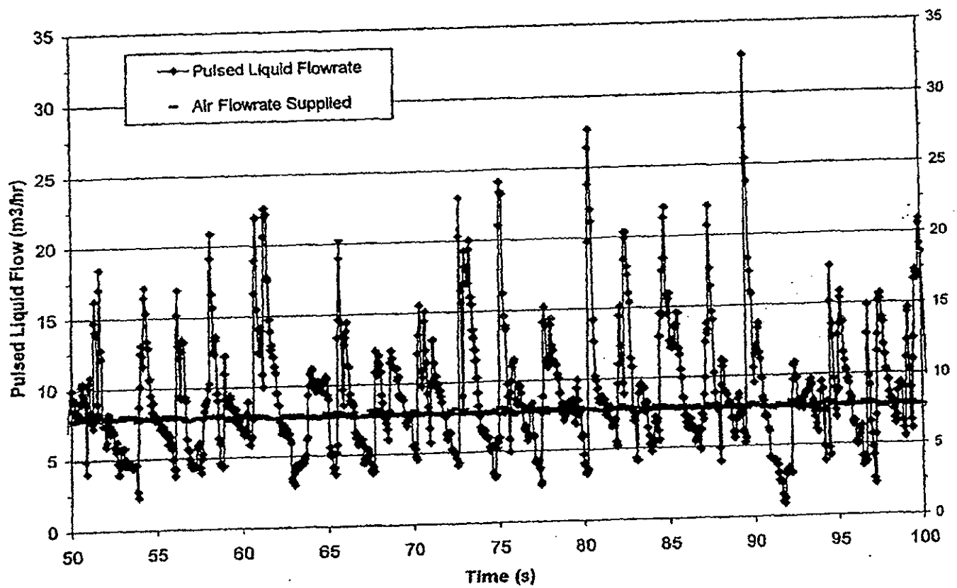
Pulsed Liquid Flow Lifted by Air
