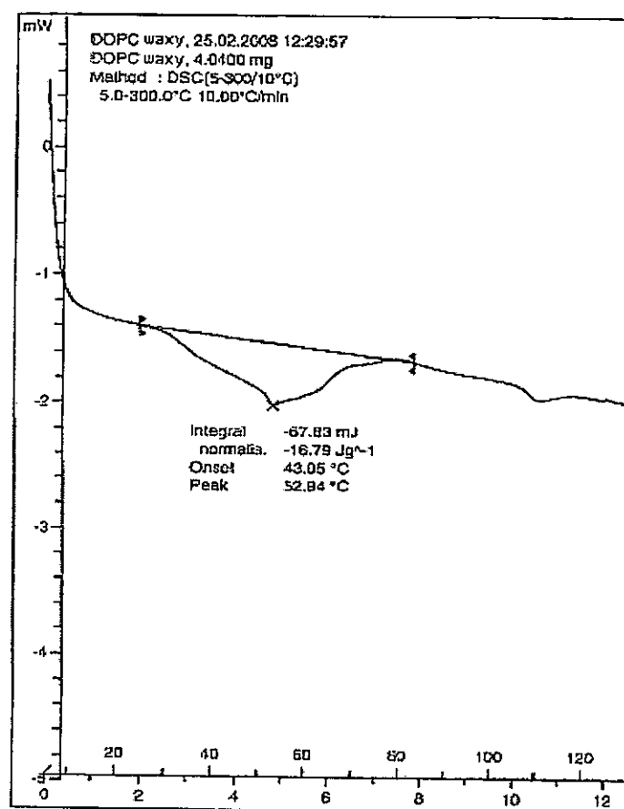
Fig. 11 (Melting behaviour of waxy DOPC)
