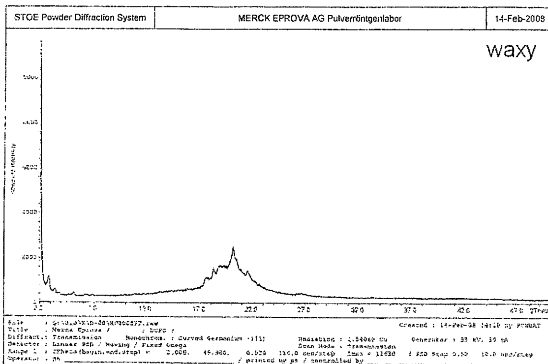
Fig. 3 (XRD spectrum of waxy DOPC)
