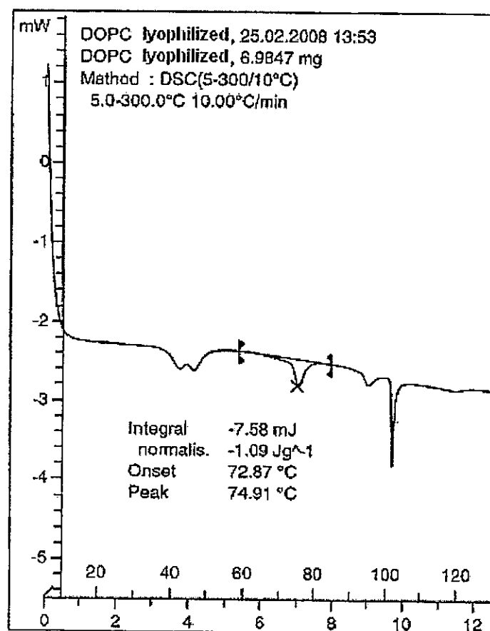
Fig. 10 (Melting behaviour of lyophilised DOPC)
