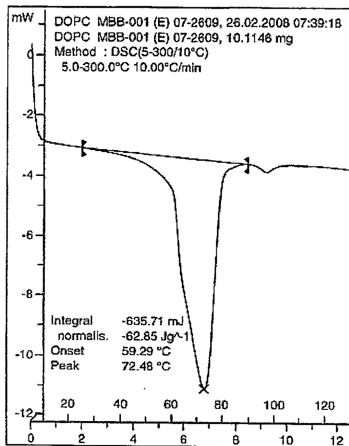
Fig. 9 (Melting behaviour of type I DOPC)
