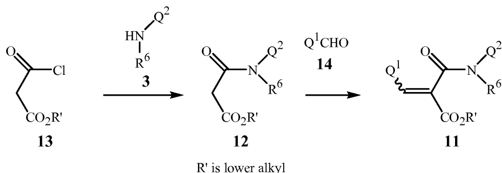
Scheme 9
