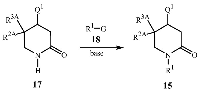
Scheme 13
