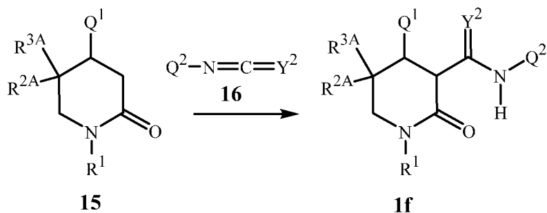
Scheme 12
