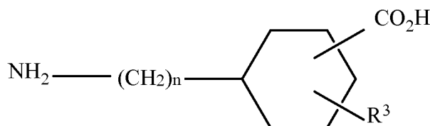
Formula (3)
