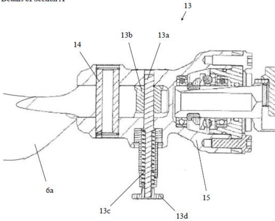
Fig. 7 Details of Section A
