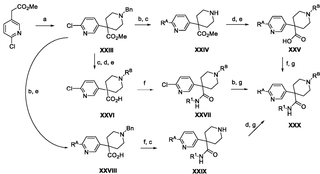
Scheme B
