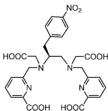
p-NO 2 -Bn-H 4 octapa
