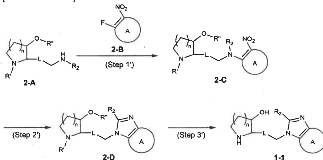
[Reaction Scheme 2]
