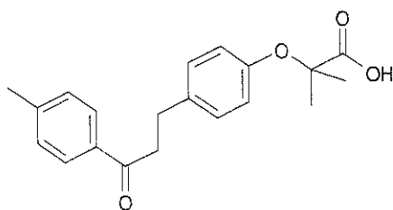
5 Compound 22 : 2-[2,6-dimethyl-4-[3-[4-(methylthio)phenyl]-3-cyclohexylmethoxypropyl]phenoxy]-2-methylpropanoic acid
