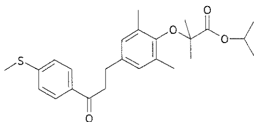
Compound 14: 2-[2,6-dimethyl-4-[3-[4-(methylthio)phenyl]-3-hydroxyimino-propyl]phenoxy]-2-methylpropanoic acid
