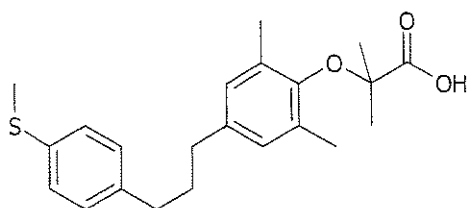
5 Compound 13: 2-[2,6-dimethyl-4-[3-[4-(methylthio)phenyl]-3-oxo-propyl]phenoxy]-2-methyl propanoic acid isopropyl ester
