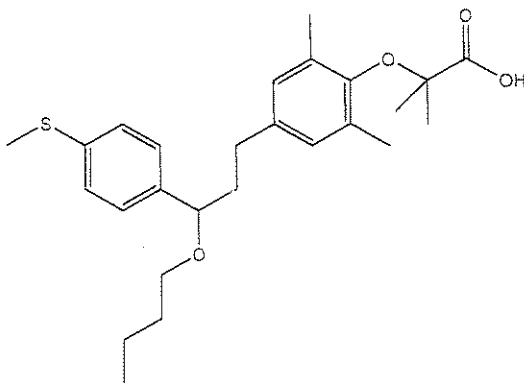
15 Compound 23 : 2-[2,6-dimethyl-4-[3-[4-(methylthio)phenyl]-3-butylmethoxypropyl]phenoxy]-2-methylpropanoic acid
