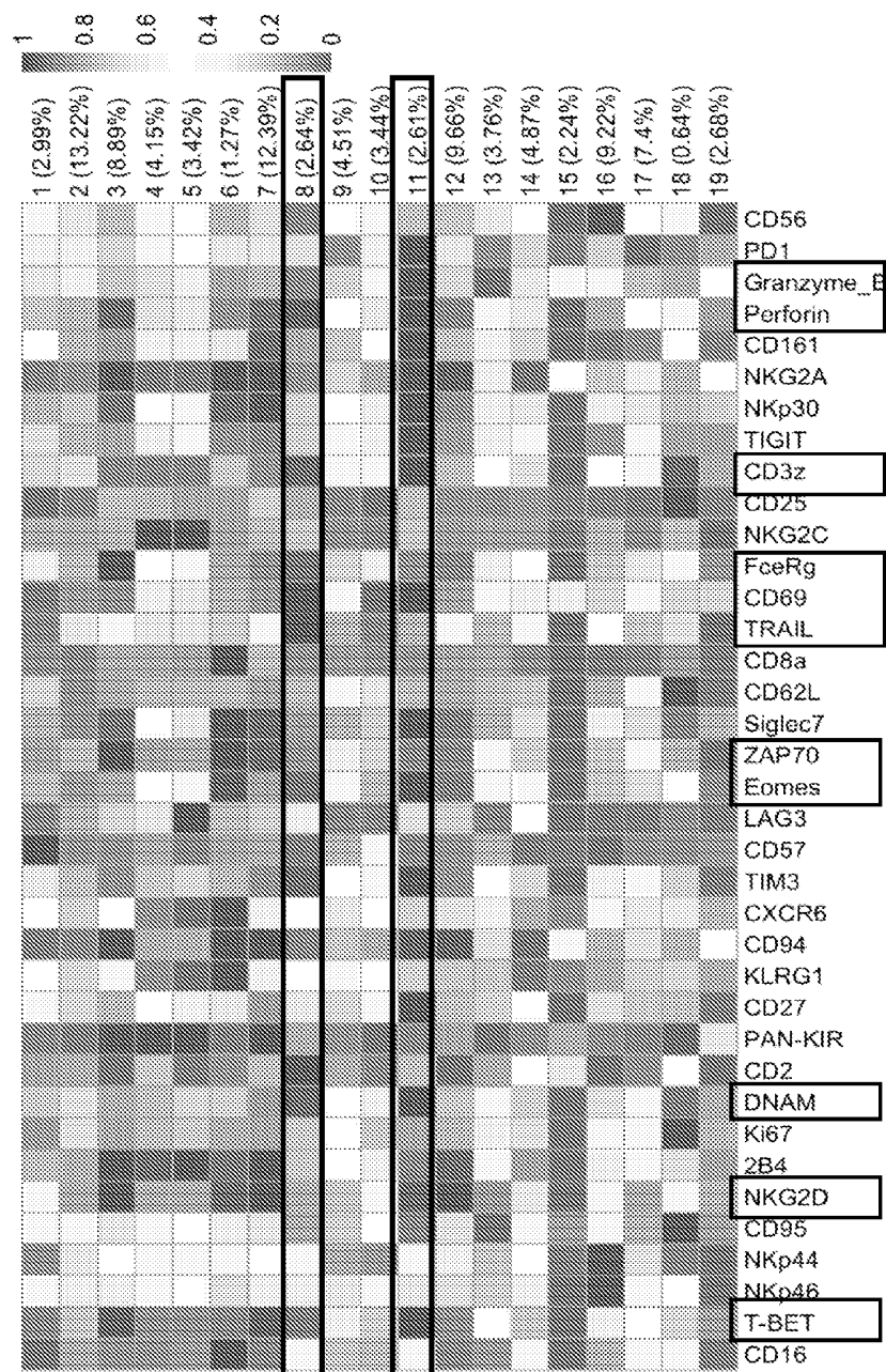
Heatmap showing normalized marker expression of each cluster
