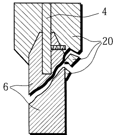
FIG. 7 PRIOR ART
