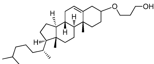
(Cholesterol),
