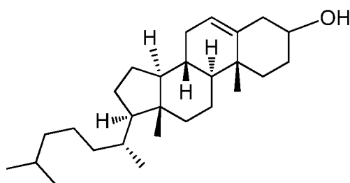
(Cholesterol),
