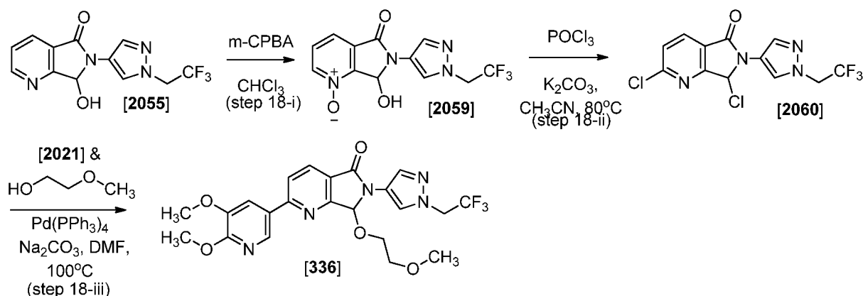
Scheme 18
