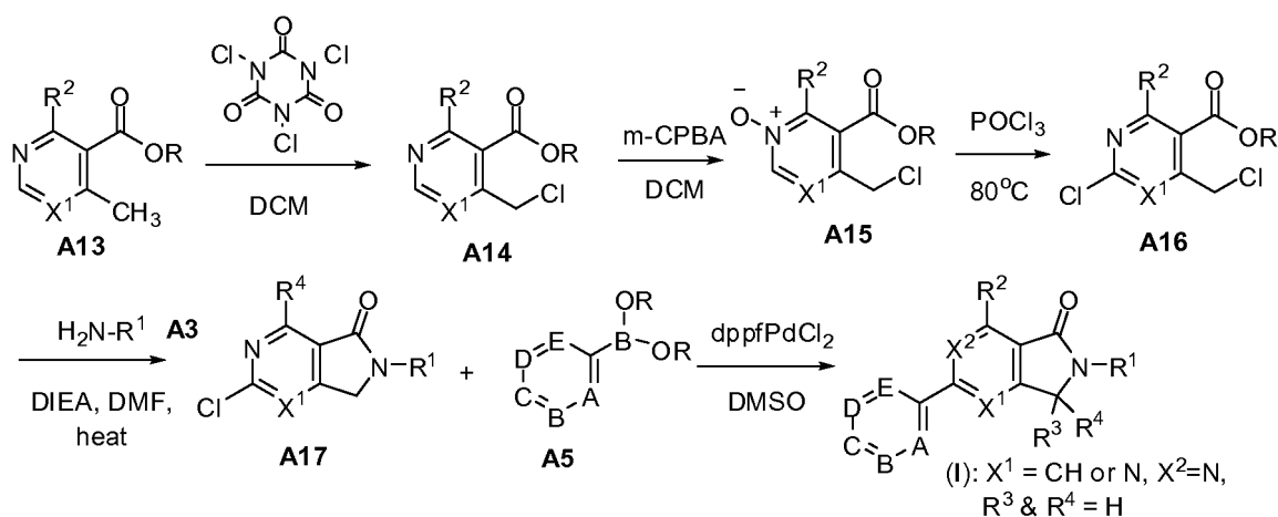
Scheme 1, Route D
