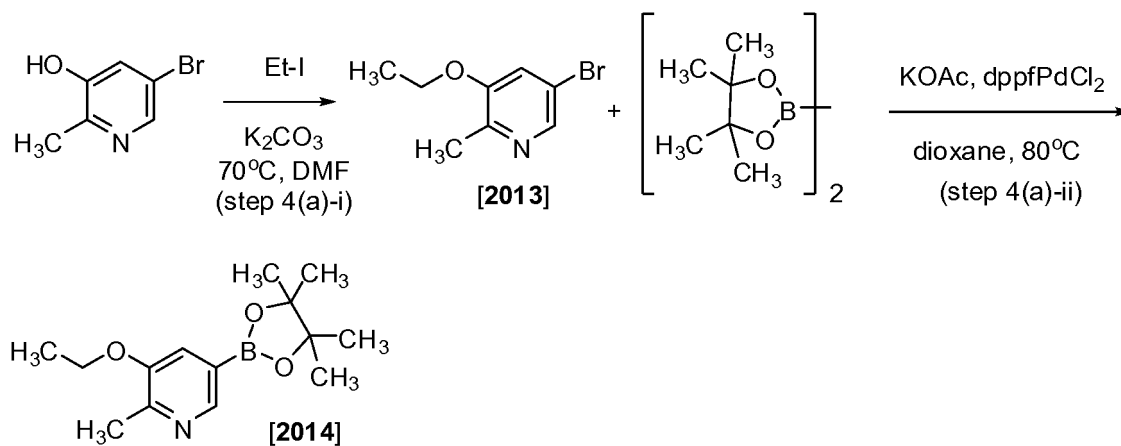
Scheme 4(a)
