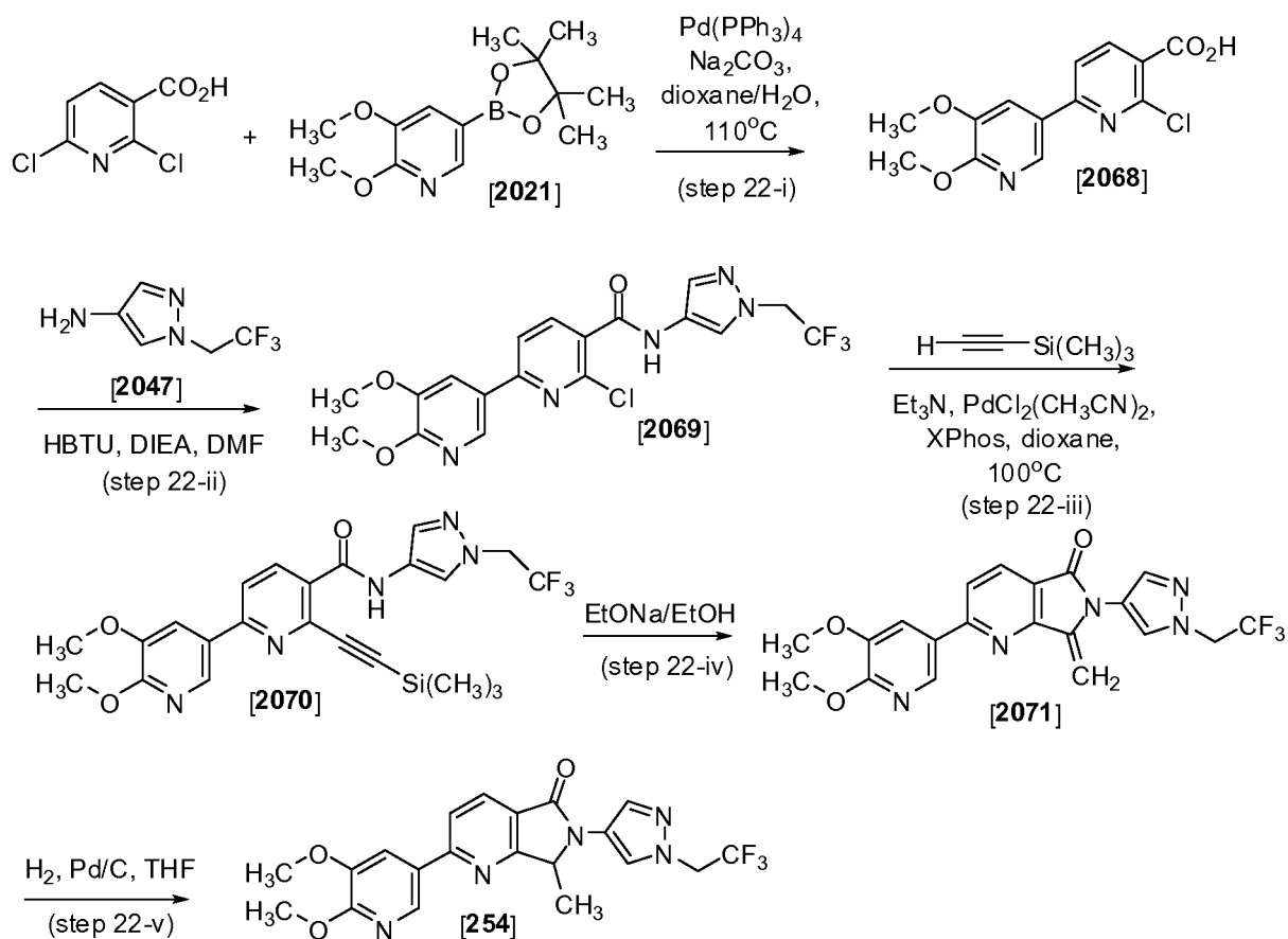
Scheme 22
