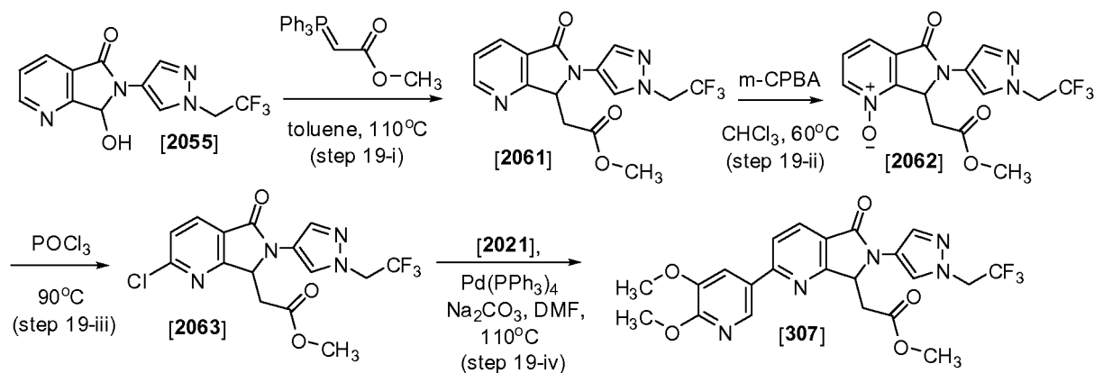
Scheme 19
