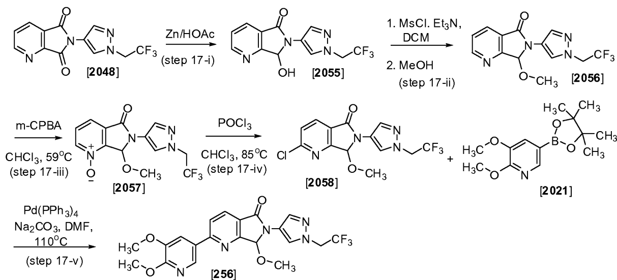
Scheme 17
