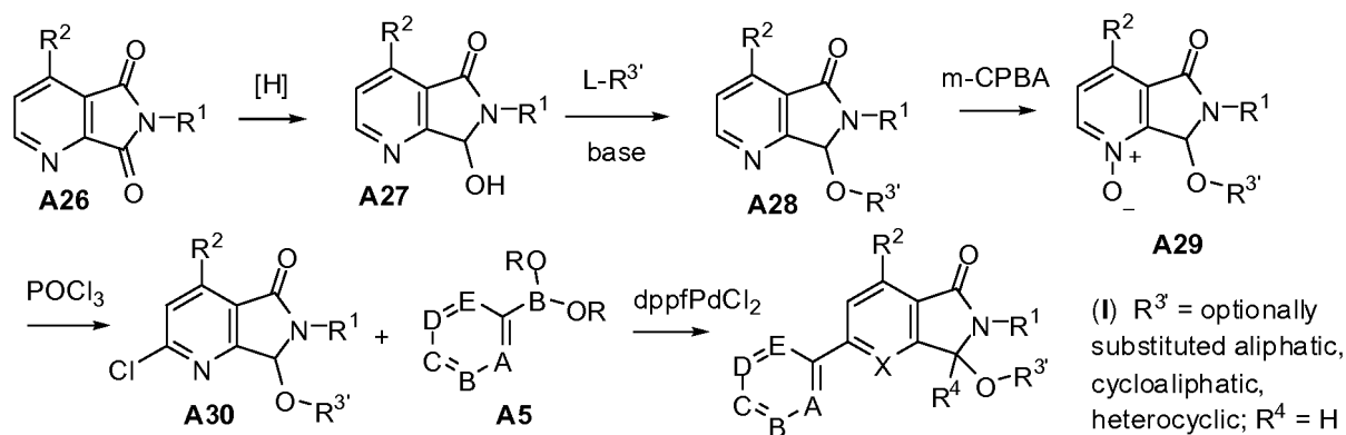
Scheme 1, Route H
