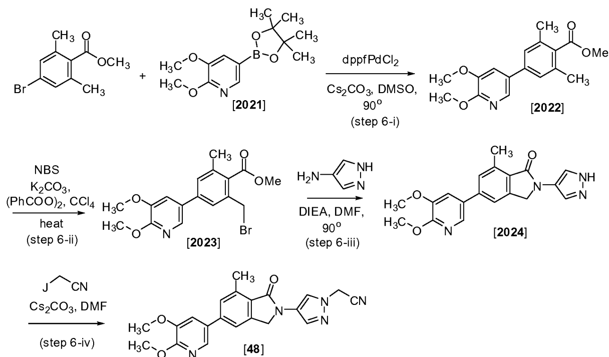
Scheme 6
