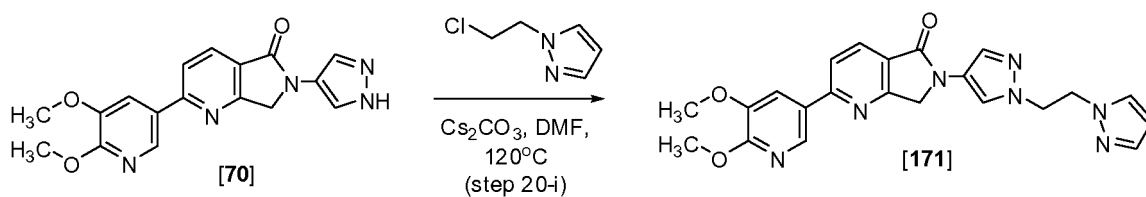
Scheme 20
