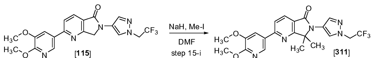
Scheme 15
