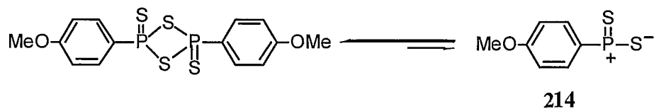
Scheme 14. The mechanism of catalysis for Lawesson's reagent.
