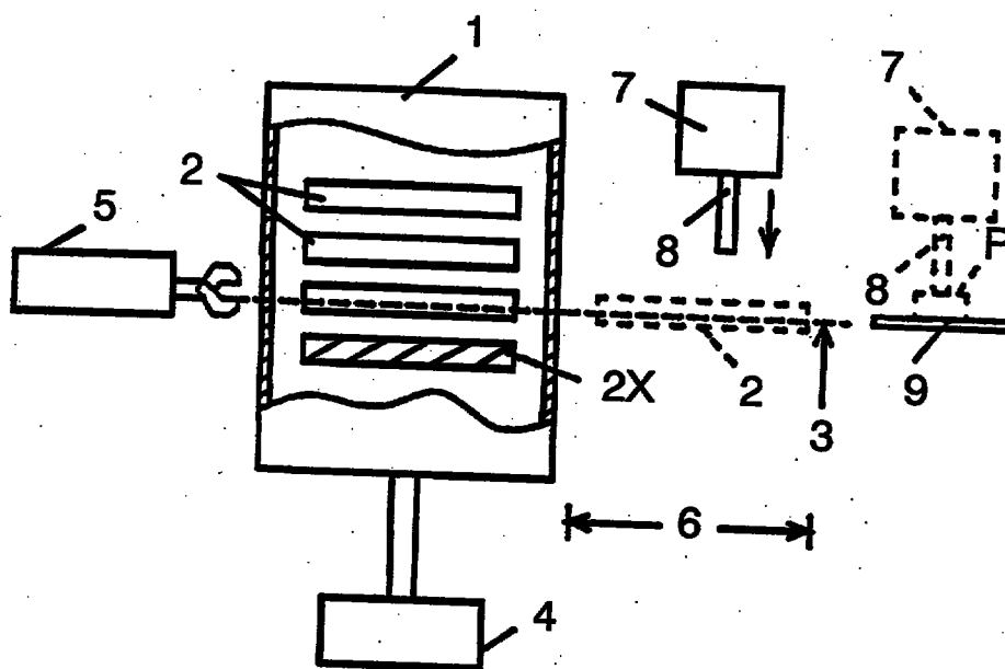
FIG. 13 PRIOR ART
