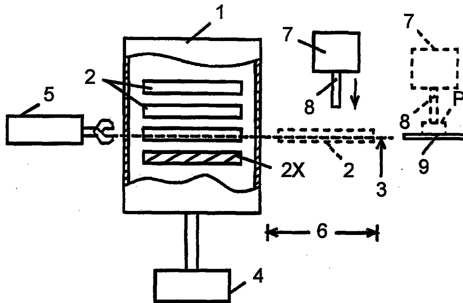
FIG. 13 PRIOR ART
