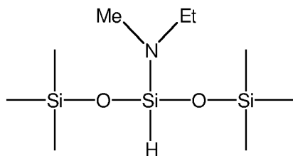
3-ethylmethylamino-1,1,1,5,5,5- hexamethyltrisiloxane
