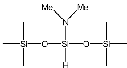
3-dimethylamino-1,1,1,5,5,5- hexamethyltrisiloxane
