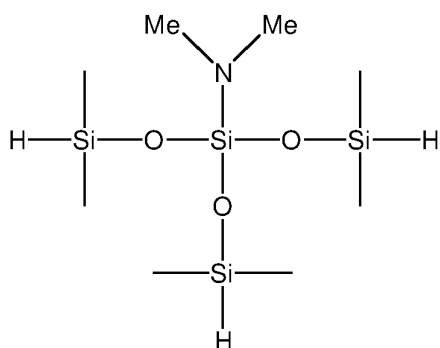
3-dimethylamino-3-(dimethylsiloxy)-1,1,5,5-tetramethyltrisiloxane
