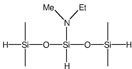
3-ethylmethylamino-1,1,5,5-tetraamethyltrisiloxane
