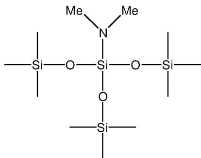
3-dimethylamino-3-(trimethylsiloxy)- 1,1,1,5,5,5-hexamethyltrisiloxane
