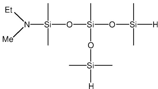
1-ethylmethylamino-3-(dimethylsiloxy)- 1,1,3,5,5-pentamethyltrisiloxane
