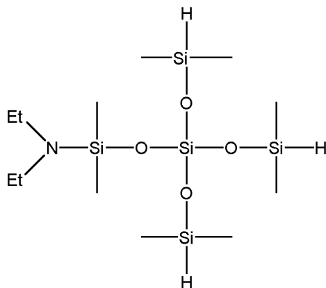
1-diethylamino-3,3-bis(dimethylsiloxy)-1,1,5,5-tetramethyltrisiloxane
