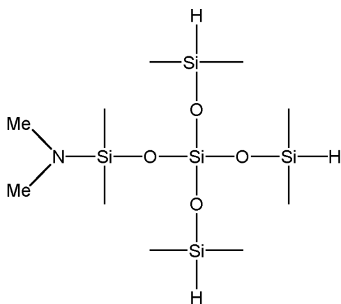
1-dimethylamino-3,3-bis(dimethylsiloxy)-1,1,5,5-tetramethyltrisiloxane
