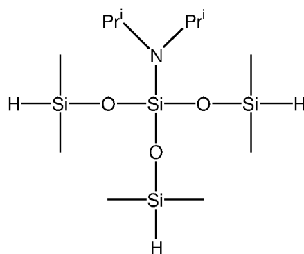
3-di-iso-propylamino-3-(dimethylsiloxy)-1,1,5,5-tetramethyltrisiloxane
