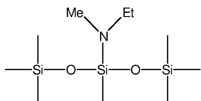
3-ethylmethylamino-1,1,1,3,5,5,5-heptamethyltrisiloxane
