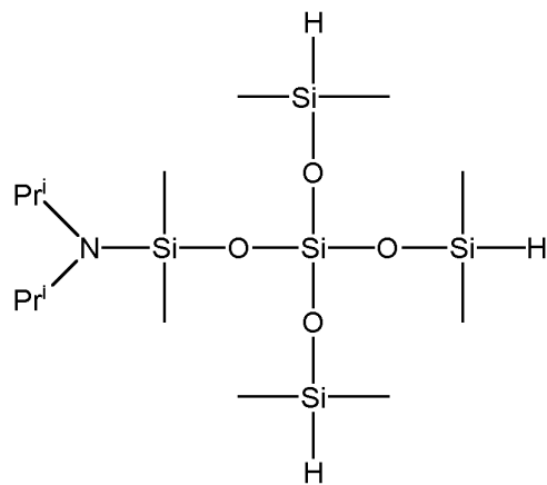
1-di-iso-propylamino-3,3-bis(dimethylsiloxy)-1,1,5,5-tetramethyltrisiloxane
