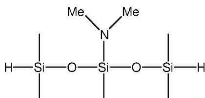
3-dimethylamino-1,1,3,5,5-pentamethyltrisiloxane
