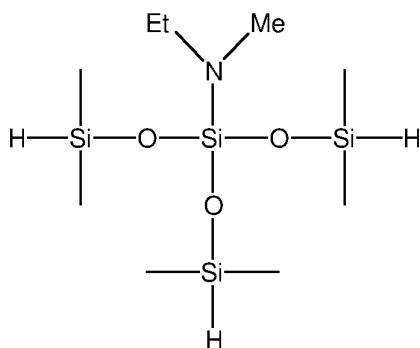
3-ethylmethylamino-3-(dimethylsiloxy)-1,1,5,5-tetramethyltrisiloxane
