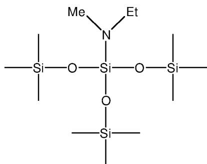
3-ethylmethylamino-3-(trimethylsiloxy)- 1,1,1,5,5,5-hexamethyltrisiloxane
