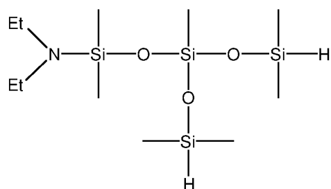
1-diethylamino-3-(dimethylsiloxy)-1,1,3,5,5-pentamethyltrisiloxane
