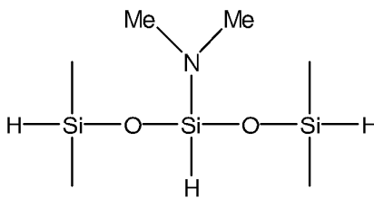
3-dimethylamino-1,1,5,5- tetramethyltrisiloxane
