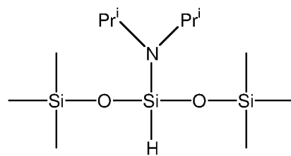
3-di-iso-propylamino-1,1,1,3,5,5,5- hexamethyltrisiloxane
