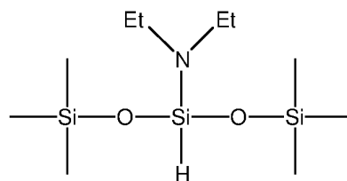
3-diethylamino-1,1,1,5,5,5- hexamethyltrisiloxane
