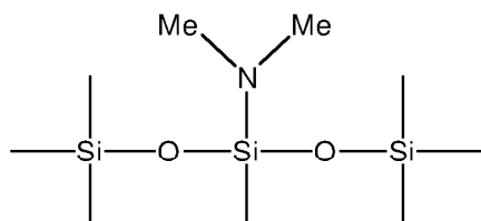
3-dimethylamino-1,1,1,3,5,5,5-heptamethyltrisiloxane
