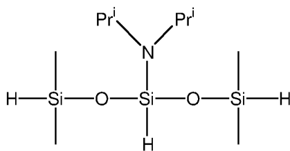
3-di-iso-propylamino-1,1,5,5-tetramethyltrisiloxane
