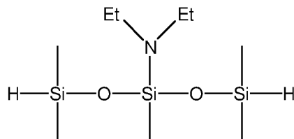
3-diethylamino-1,1,3,5,5-pentamethyltrisiloxane
