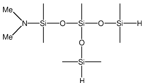
1-dimethylamino-3-(dimethylsiloxy)-1,1,3,5,5-pentamethyltrisiloxane
