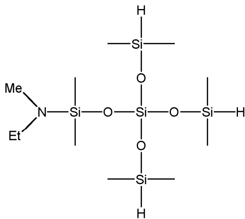
1-ethylmethylamino-3,3-bis(dimethylsiloxy)-1,1,5,5-tetramethyltrisiloxane
