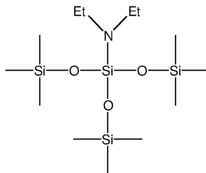
3-diethylamino-3-(trimethylsiloxy)-1,1,1,5,5,5- hexamethyltrisiloxane
