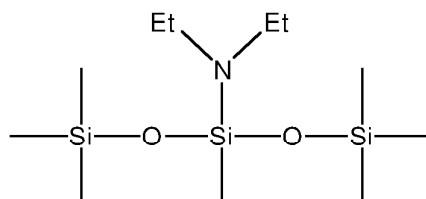
3-diethylamino-1,1,1,3,5,5,5-heptamethyltrisiloxane
