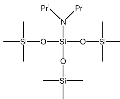
3-di-iso-propylamino-3-(trimethylsiloxy)- 1,1,1,5,5,5-hexamethyltrisiloxane
