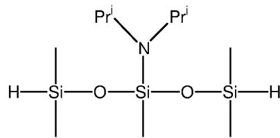
3-di-iso-propylamino-1,1,3,5,5-pentamethyltrisiloxane
