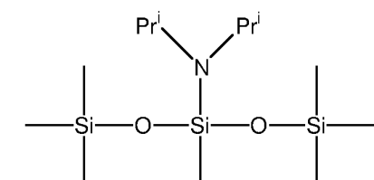
3-di-iso-propylamino-1,1,1,3,5,5,5-heptamethyltrisiloxane
