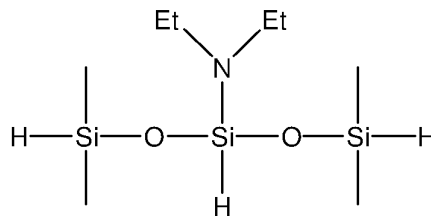
3-diethylamino-1,1,5,5-tetramethyltrisiloxane
