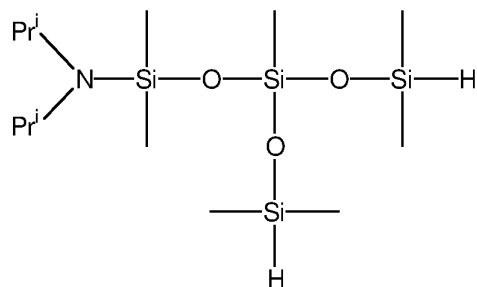
1-di-iso-propylamino-3-(dimethylsiloxy)- 1,1,3,5,5-pentamethyltrisiloxane
