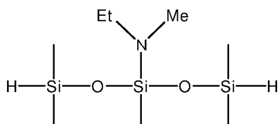
3-ethylmethylamino-1,1,3,5,5-pentamethyltrisiloxane
