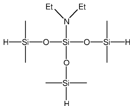
3-diethylamino-3-(dimethylsiloxy)-1,1,5,5-tetramethyltrisiloxane
