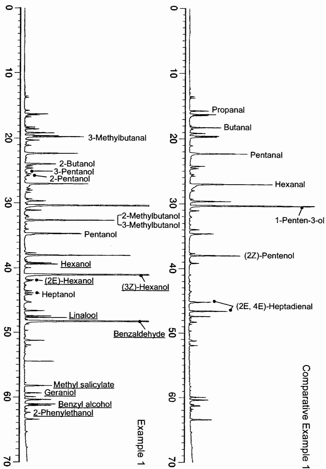
Fig. 1 Gas Chromatogram of Head Space Analysis
