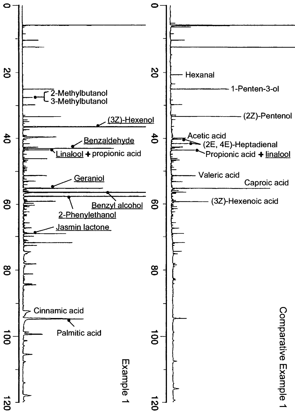
Fig. 2 Gas Chromatogram of Flavor Condensate Obtained by Ether Extraction
