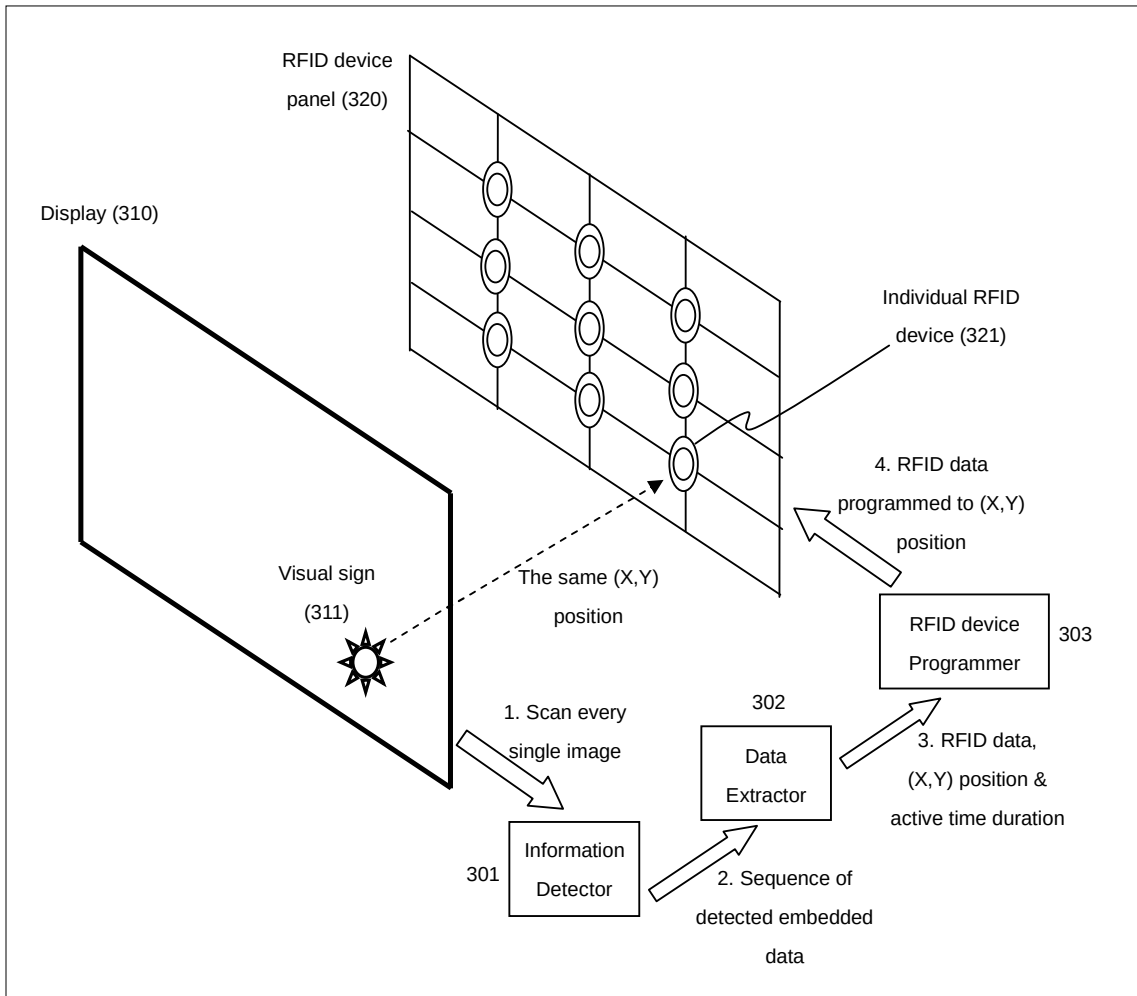
FIGURE 3: System design
