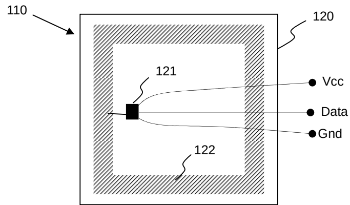
FIGURE 1: RFID Tag
