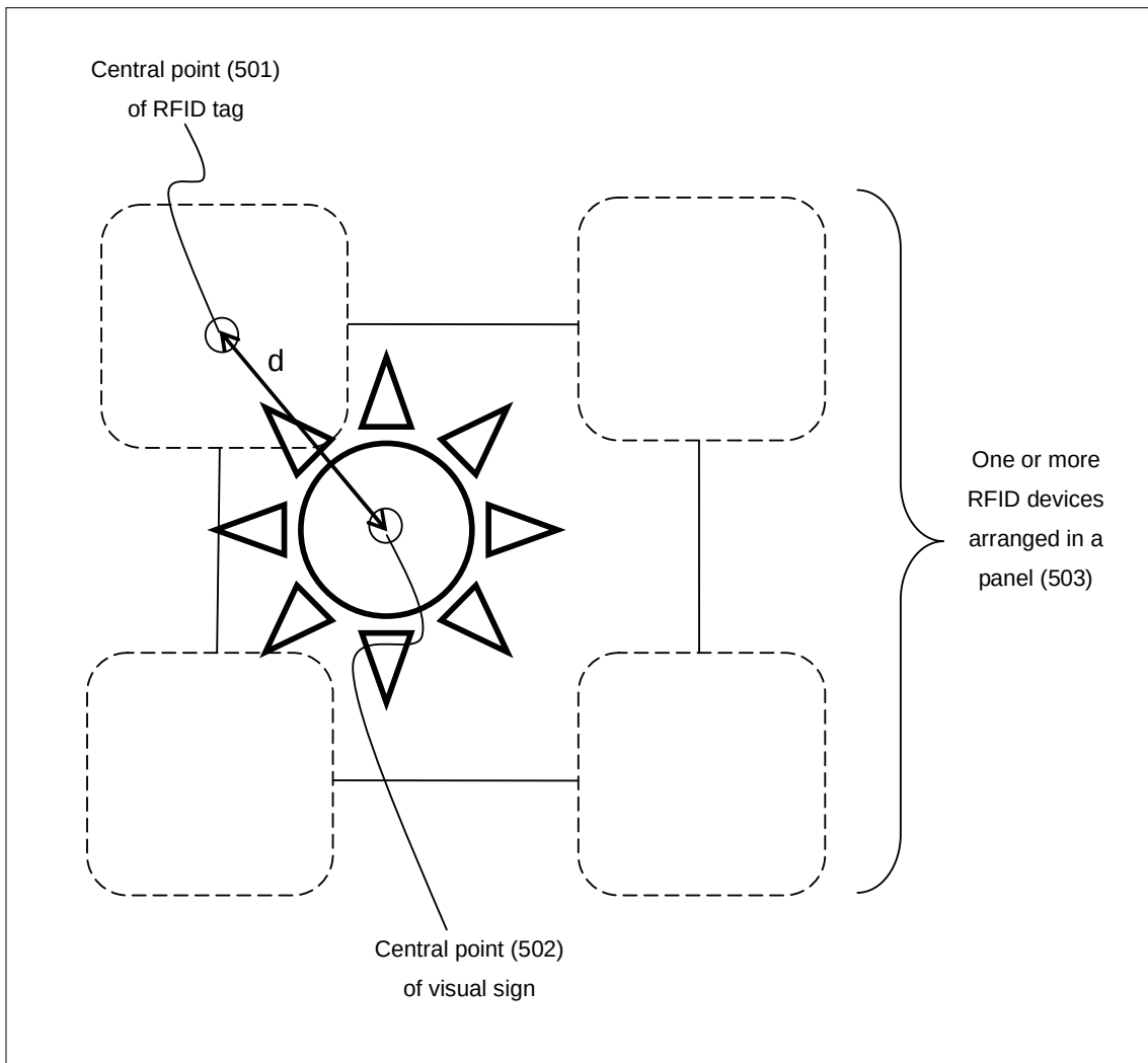
FIGURE 5: The visual sign is surrounded by more than one RFID tags
