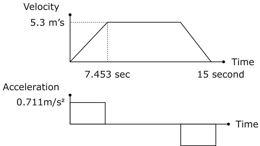
Fig. 25(a) Cage acceleration and speed
