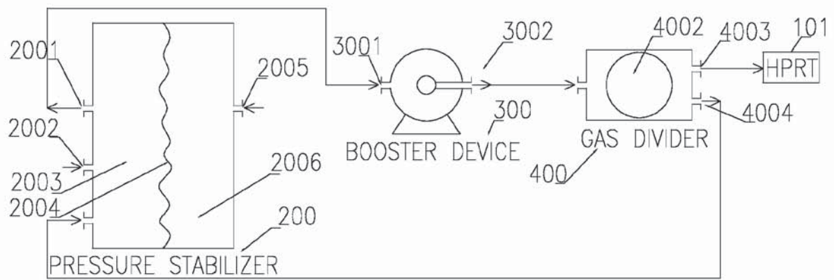
(FIGURE 8) POSITIVE TYPE CONNECTION WITH GAS REFLUX LOOP
