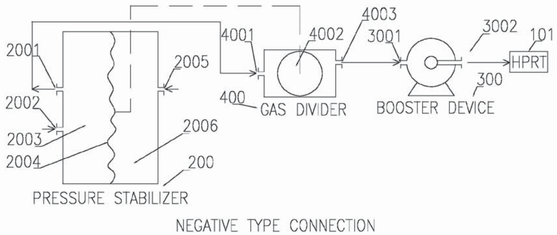
(FIGURE 1) TWO TYPE PPSS CONNECTION
