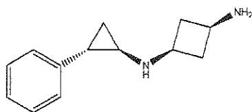
Example 88: ( trans )-N1-((1 S ,2 R )-2-phenylcyclopropyl)cyclobutane-1,3-diamine
