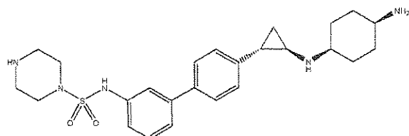
10 Example 104: N-(4'-((1 R ,2 S )-2-((( trans )-4-aminocyclohexyl)amino)cyclopropyl)-[1,1'-biphenyl]-3-yl)piperazine-1-sulfonamide
