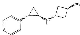
Example 87: ( cis )-N1-((1 R ,2 S )-2-phenylcyclopropyl)cyclobutane-1,3-diamine
