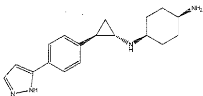
Example 98: ( trans )-N1-((1 R ,2 S )-2-(4-(1H-pyrazol-5-yl)phenyl)cyclopropyl)cyclohexane-1,4-diamine
