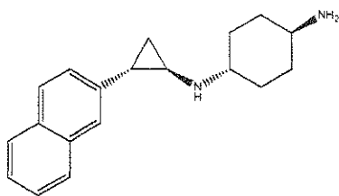
Example 95: ( cis )-N1-((1 R ,2 S )-2-(naphthalen-2-yl)cyclopropyl)cyclohexane-1,4-diamine
