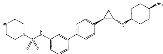
5 Example 102: N-(4'-((1 S ,2 R )-2-((( trans )-4-aminocyclohexyl)amino)cyclopropyl)-[1,1'-biphenyl]-3-yl)piperazine-1-sulfonamide
