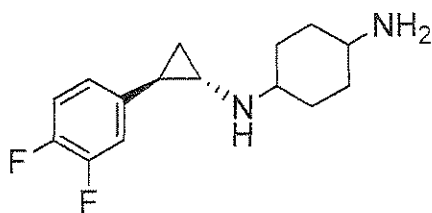
Example 80: N1-(( trans )-2-methyl-2-phenylcyclopropyl)cyclohexane-1,4-diamine
