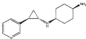
Example 82: ( trans )-N1-((1 R ,2 S )-2-(pyridin-3-yl)cyclopropyl)cyclohexane-1,4-diamine
