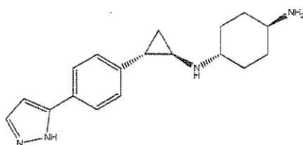
Example 99: ( cis )-N1-((1 R ,2 S )-2-(4-(1H-pyrazol-5-yl)phenyl)cyclopropyl)cyclohexane-1,4-diamine
