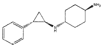
Example 83: ( cis )-N1-((1 R ,2 S )-2-(pyridin-3-yl)cyclopropyl)cyclohexane-1,4-diamine
