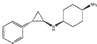
Example 84: ( trans )-N1-((1 S ,2 R )-2-(pyridin-3-yl)cyclopropyl)cyclohexane-1,4-diamine
