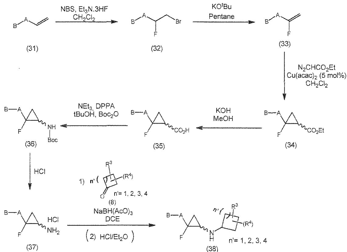
SCHEME 6: Boc 2 O (Di- tert -butyl dicarbonate), DCE (Dichloroethane), DPPA (Diphenylphosphoryl azide), Cu(acac) 2 (Copper(II) acetylacetonate), NBS (N-Bromosuccinimide).
