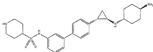
Example 103: N-(4'-((1 S ,2 R )-2-((( cis )-4-aminocyclohexyl)amino)cyclopropyl)-[1,1'-biphenyl]-3-yl)piperazine-1-sulfonamide
