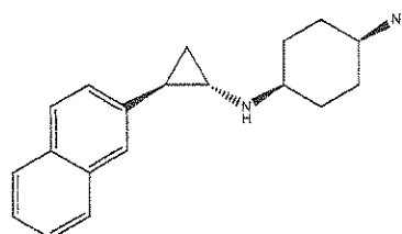
Example 94: ( trans )-N1-((1 R ,2 S )-2-(naphthalen-2-yl)cyclopropyl)cyclohexane-1,4-diamine
