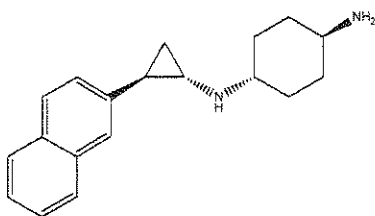
Example 97: ( cis )-N1-((1 S ,2 R )-2-(4-(1H-pyrazol-5-yl)phenyl)cyclopropyl)cyclohexane-1,4-diamine
