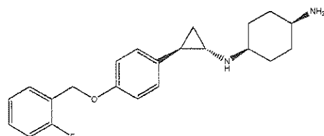
15 Example 106: ( trans )-N1-((1 R ,2 S )-2-(4-((2-fluorobenzyl)oxy)phenyl)cyclopropyl)cyclohexane-1,4-diamine
