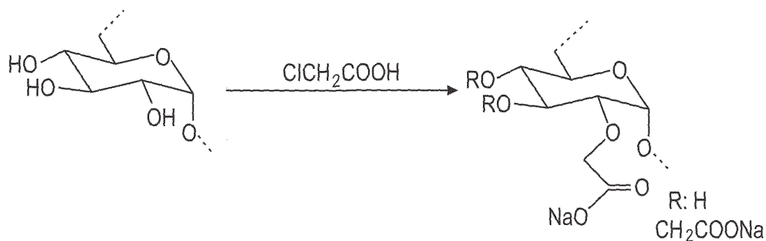
Reaction scheme 2
