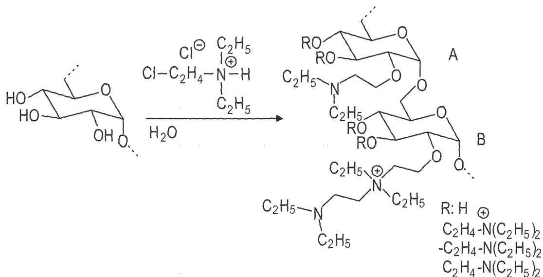
Reaction scheme 1: DEAE dextran containing 2-(diethylamino)ethyl (A) and 2-[(2-(diethylamino)ethyl)diethylammonium]ethyl (B) groups
