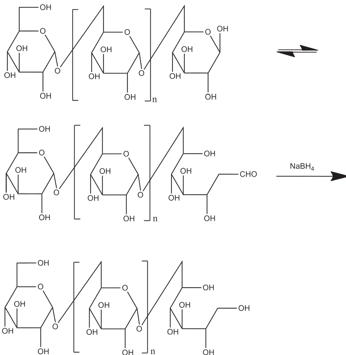
Reaction scheme 4
