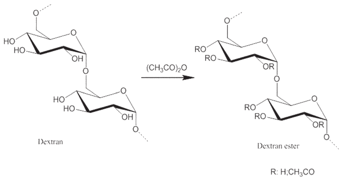
Reaction scheme 3
