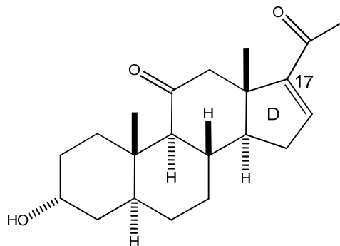
Compound B
