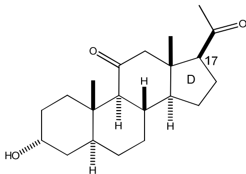
Compound A
