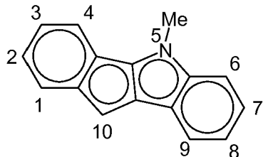
5-methylindeno[1,2- b ]indolyl
