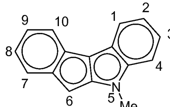
5-methylindeno[2,1- b ]indolyl
