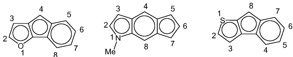
indeno[1,2- b ]furyl 1-methylcyclopenta[ f ]indolyl indeno[2,1- b ]thienyl
