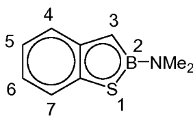
2-dimethylamino- 1,2-benzothiaborollide
