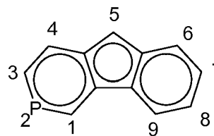
indeno[1,2-c]phosphinyl
