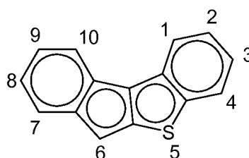
indeno[2,1- b ][1]benzothienyl
