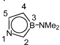
3-dimethylamino- 1,3-azaborollide
