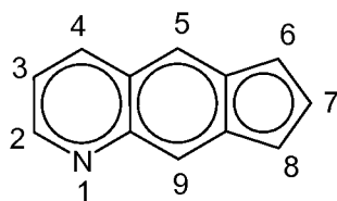
cyclopenta[g]quinolyl
