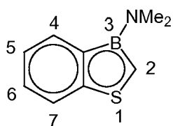
3-dimethylamino- 1,3-benzothiaborollide
