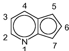
cyclopenta[b]pyridyl
