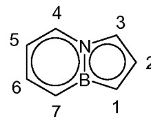
3a,7a-azaborindenyl
