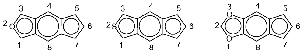
indeno[5,6- c ]furyl indeno[5,6- c ]thienyl indeno[5,6- d ][1,3]dioxolyl
