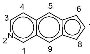
cyclopenta[g]isoquinolyl
