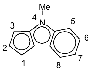
4-methylcyclopenta[ b ]indolyl
