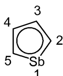
stibacyclopentadienyl
