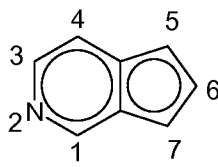
cyclopenta[c]pyridyl
