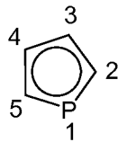
phosphacyclopentadienyl
