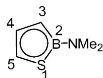
2-dimethylamino- 1,2-thiaborollide
