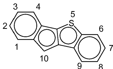
indeno[1,2- b ][1]benzothienyl
