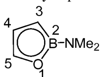
2-dimethylamino- 1,2-oxaborollide
