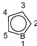
boracyclopentadienyl
