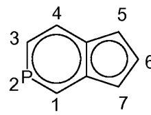
cyclopenta[c]phosphinyl
