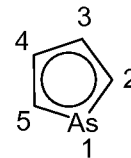
arsacyclopentadienyl
