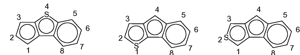
cyclopenta[ b ][1]benzothienyl indeno[1,2- b ]thienyl indeno[1,2- c ]thienyl
