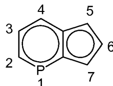
cyclopenta[b]phosphinyl
