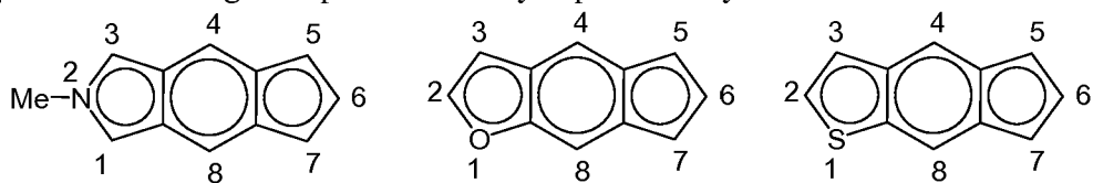
2-methylcyclopenta[ f ]isoindolyl indeno[5,6- b ]furyl indeno[5,6- b ]thienyl
