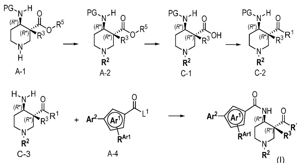
Reaction Scheme C
