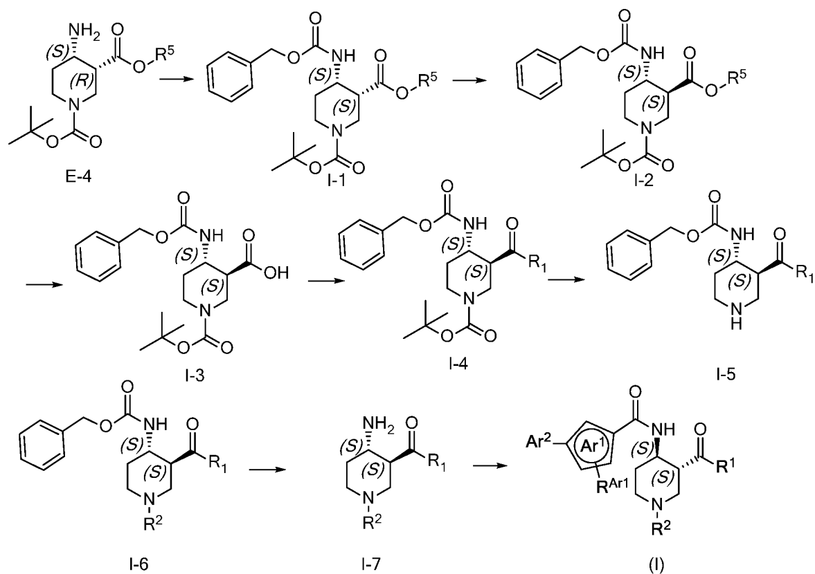
Reaction Scheme I
