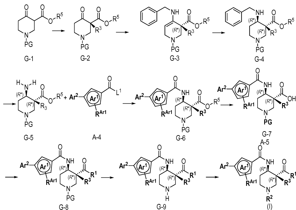
Reaction Scheme G
