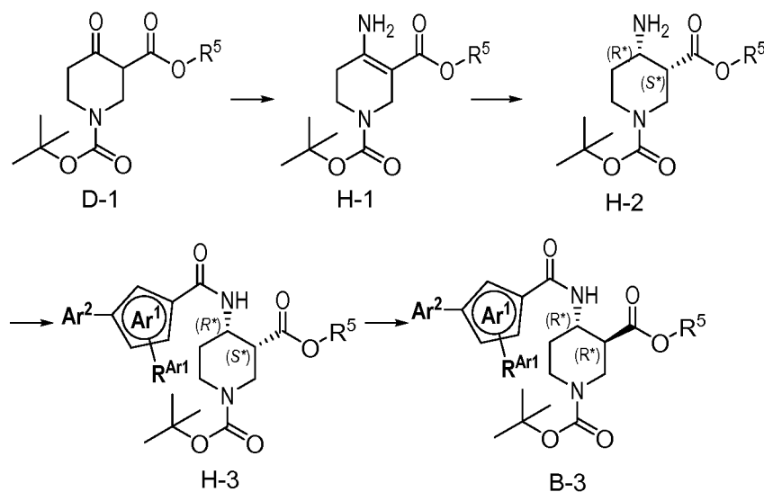
Reaction Scheme H
