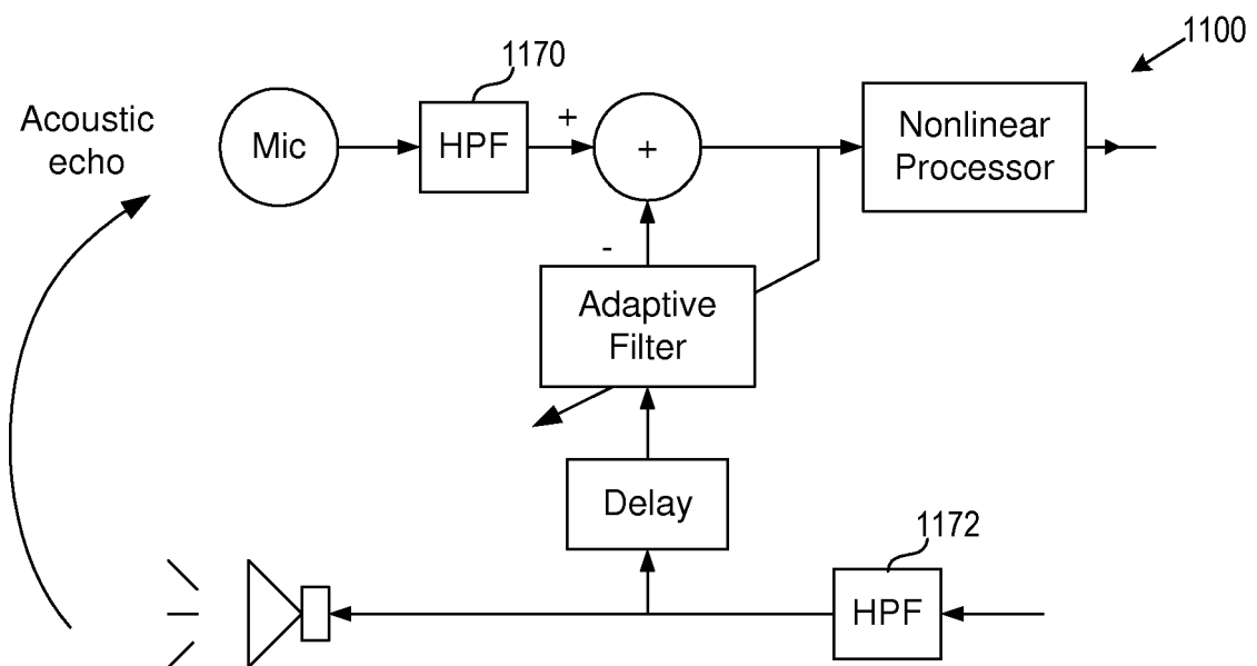
Figure 11 (PRIOR ART)
