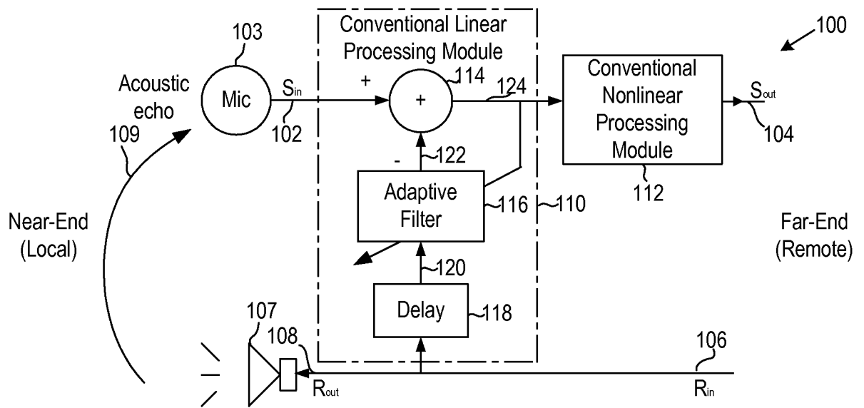
Figure 1 (PRIOR ART)
