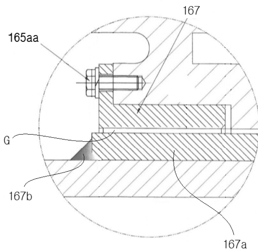
Detail of "A" Scale 5 : 1
