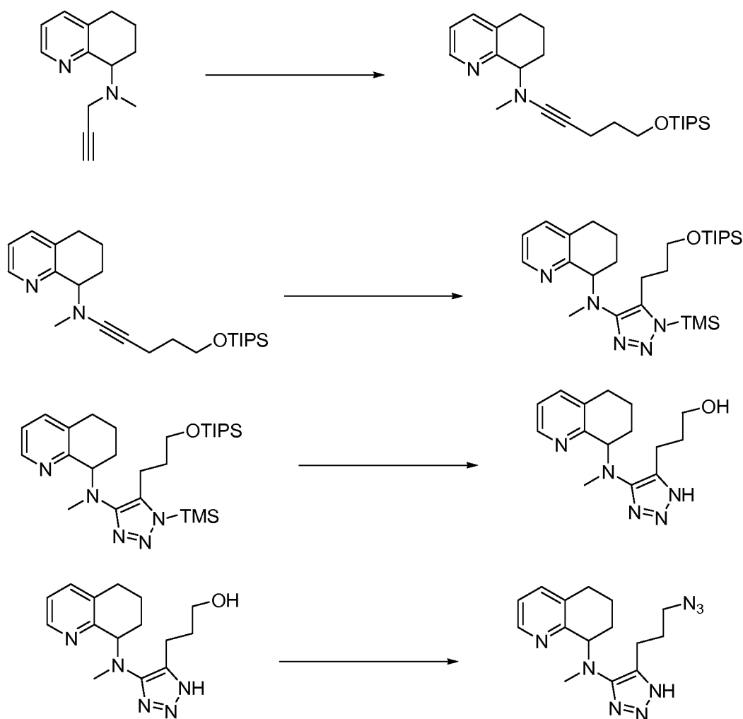
SCHEME 14
